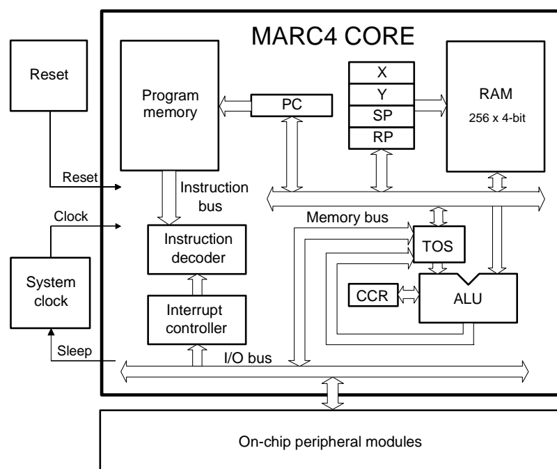
Figure 10. MARC4 Core
