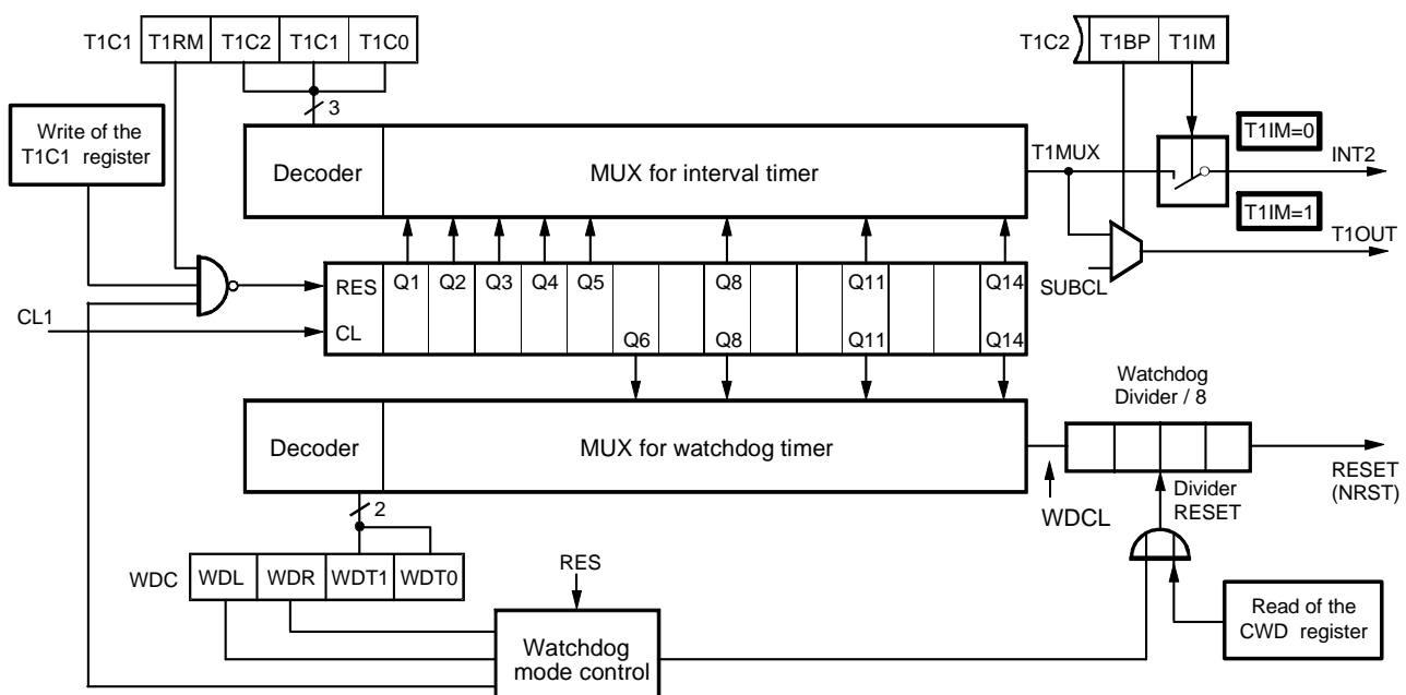
Figure 35. Timer 1 and Watchdog
