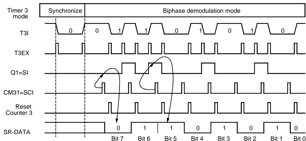
Figure 84. Biphase Demodulation
