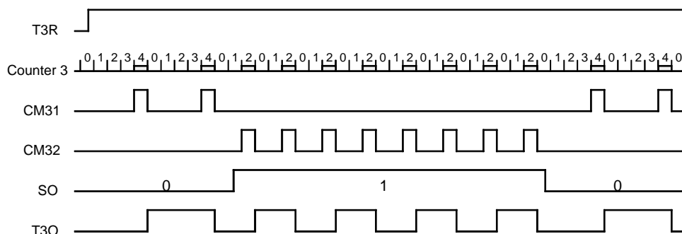
Figure 81. FSK Modulation
