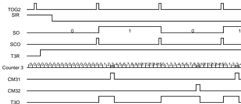
Figure 82. Pulse-width Modulation
