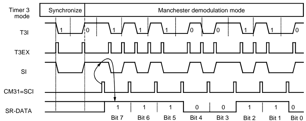
Figure 83. Manchester Demodulation
