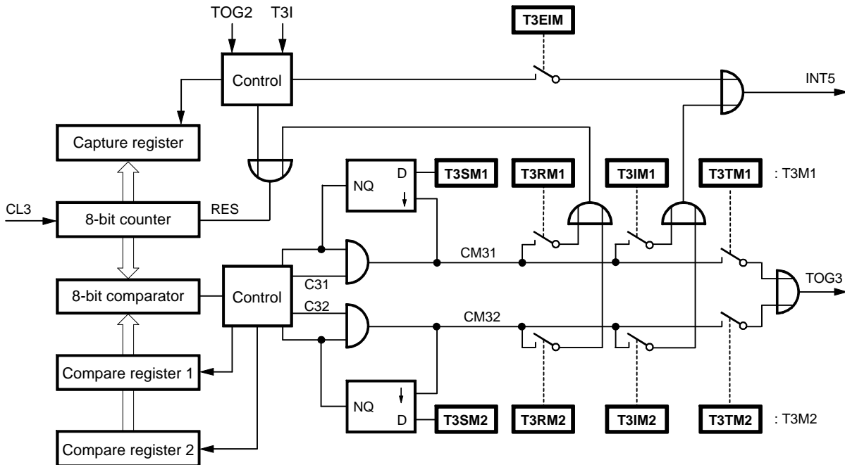
Figure 51. Counter 3 Stage
