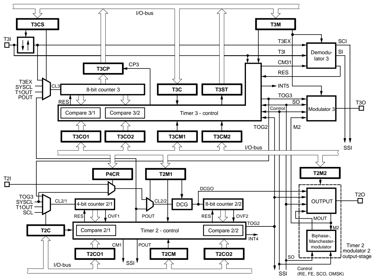
Figure 85. Combination Timer 3 and Timer 2
