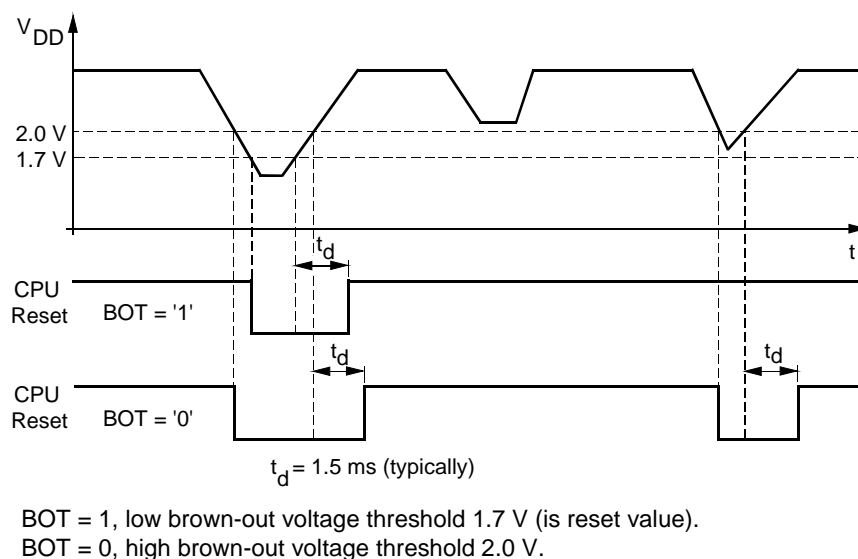
Figure 17. Brown-out Detection
