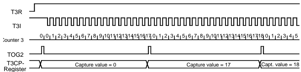
Figure 86. Frequency Measurement
