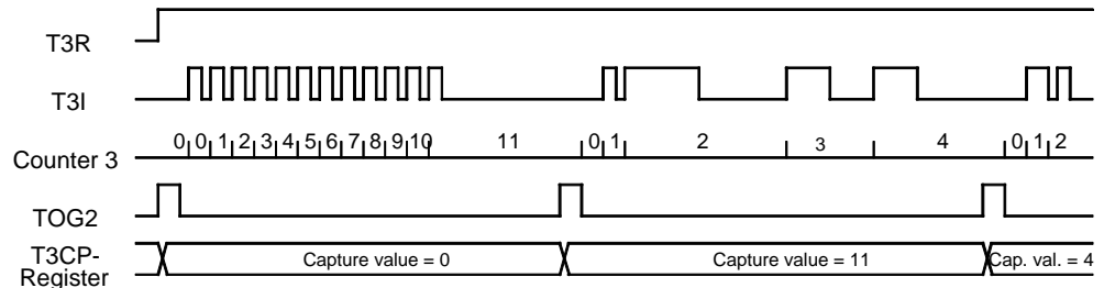
Figure 87. Event Counter with Time Gate
