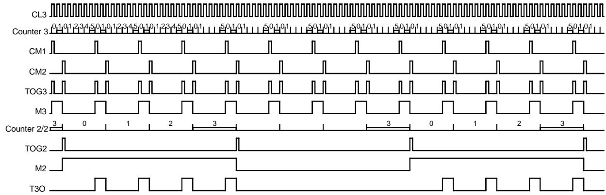
Figure 88. Burst Modulation 1
