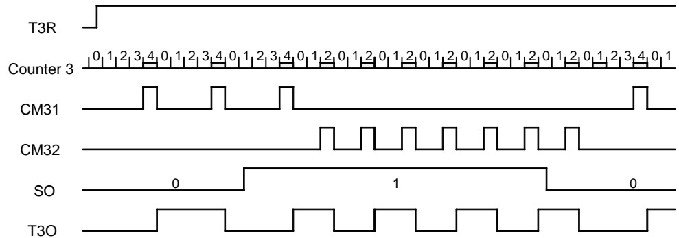
Figure 91. FSK Modulation
