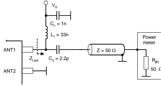
Figure 5. Output Power Measurement
