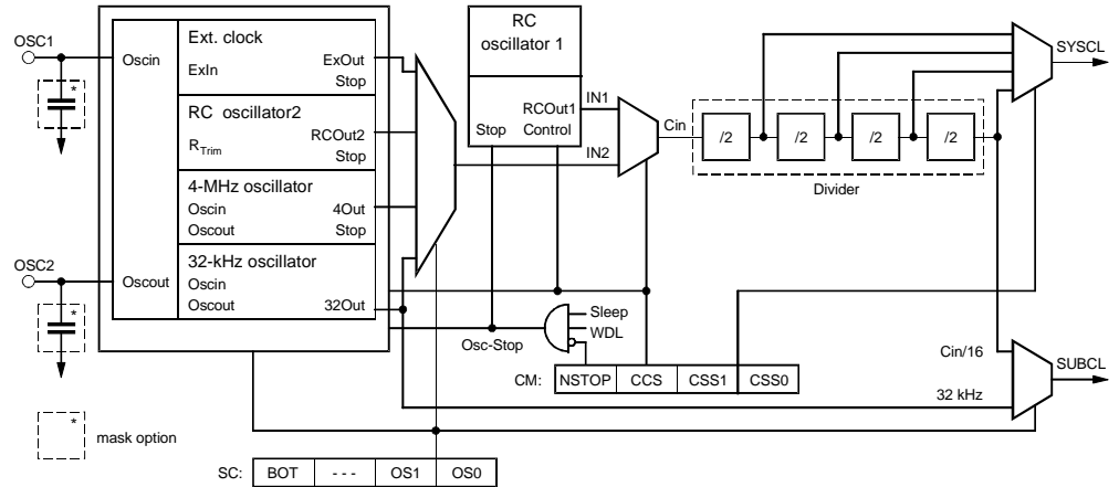
Figure 21. Clock Module
