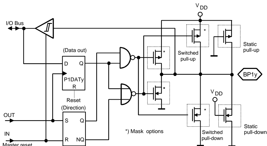
Figure 28. Bi-directional Port 1
