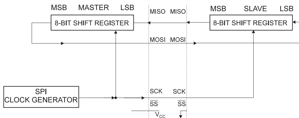
Figure 41. SPI Master-Slave Interconnection
