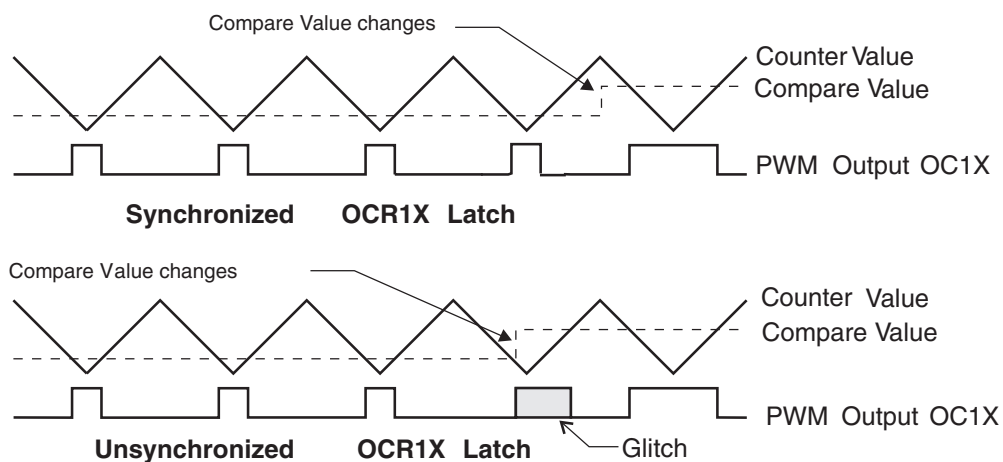
Figure 37. Effects on Unsynchronized OCR1 Latching (1)
