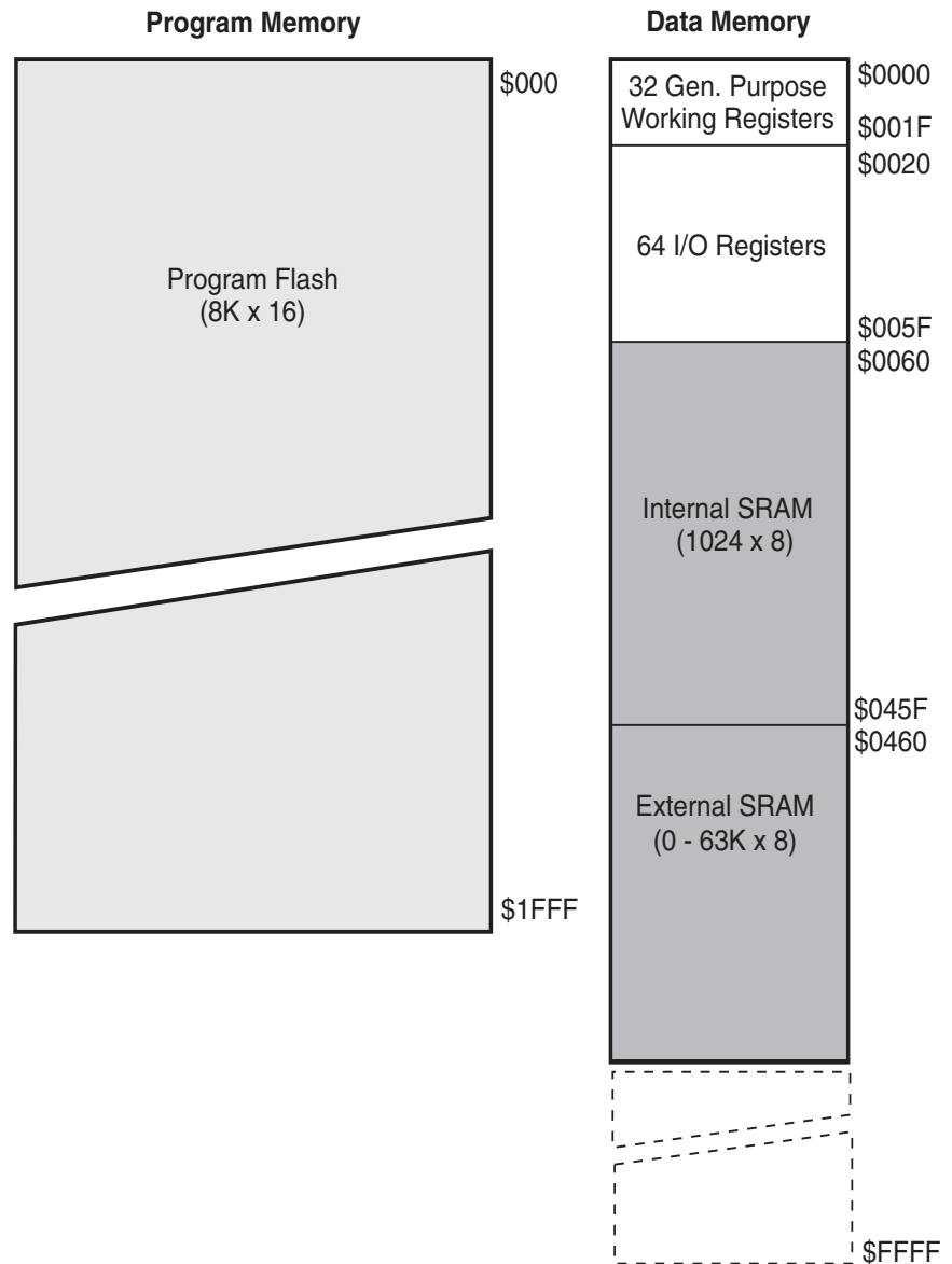
Figure 5. Memory Maps
