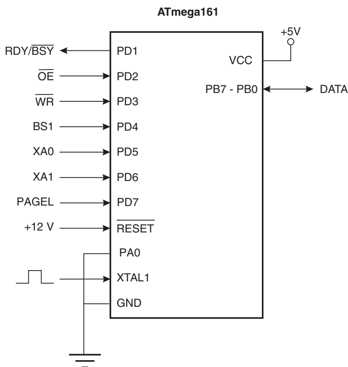
Figure 75. Parallel Programming
