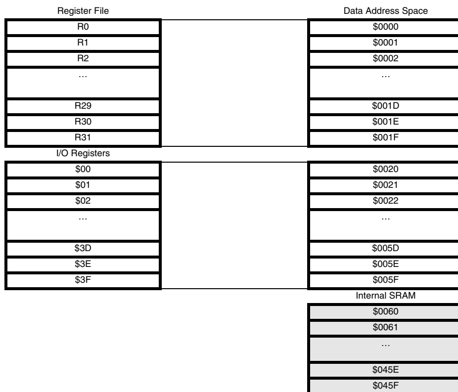
Figure 8. SRAM Organization
