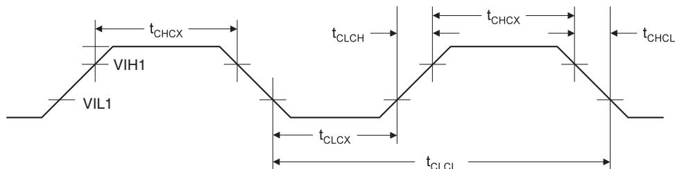
Figure 82. External Clock
