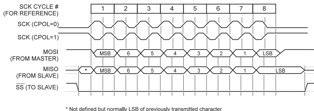
Figure 43. SPI Transfer Format with CPHA = 1 and DORD = 0
