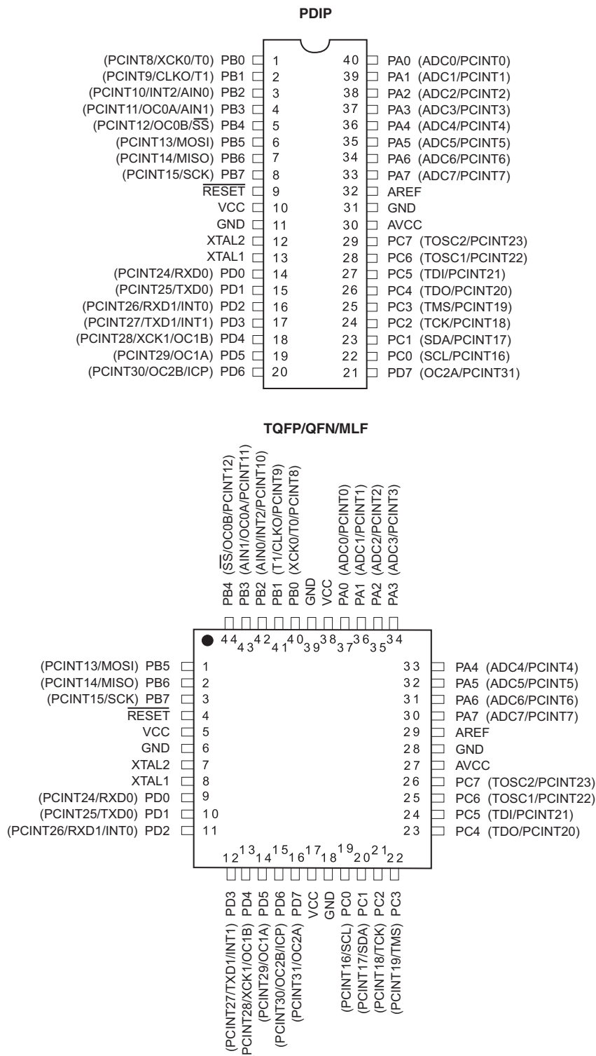
Figure 1-1. Pinout ATmega164P/324P/644P
