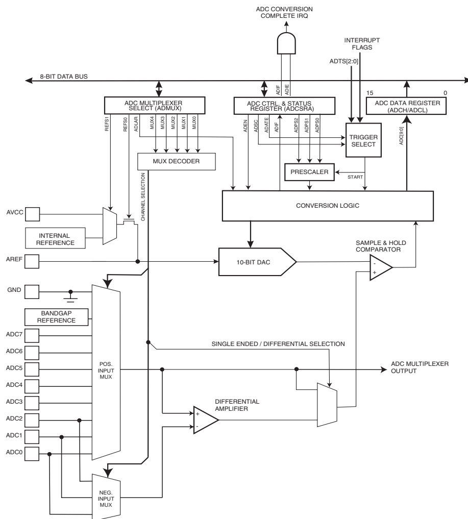
Figure 83. Analog to Digital Converter Block Schematic
