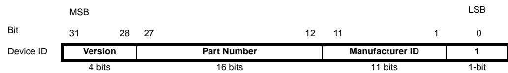
Figure 107. The Format of the Device Identification Register
