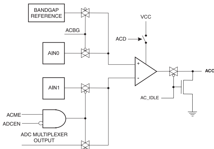
Figure 113. Analog Comparator
