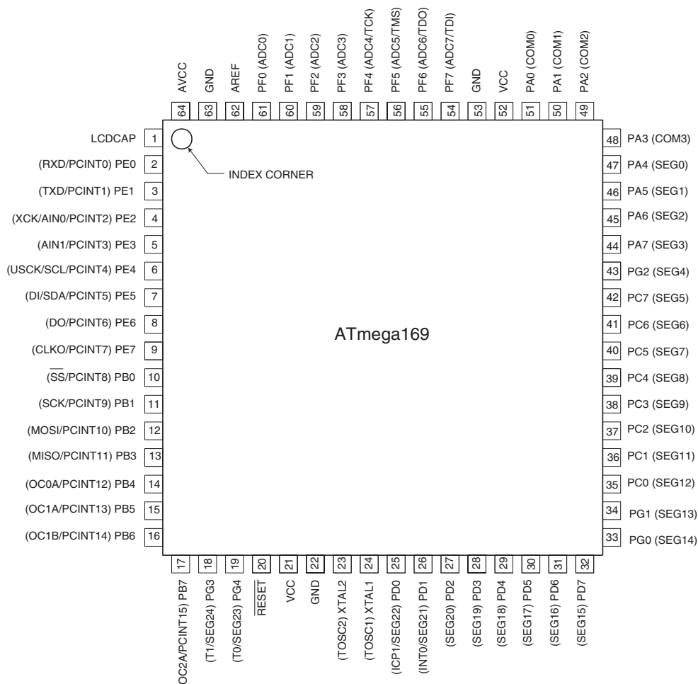
Figure 1. Pinout ATmega169
