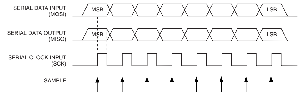
Figure 129. Serial Programming Waveforms
