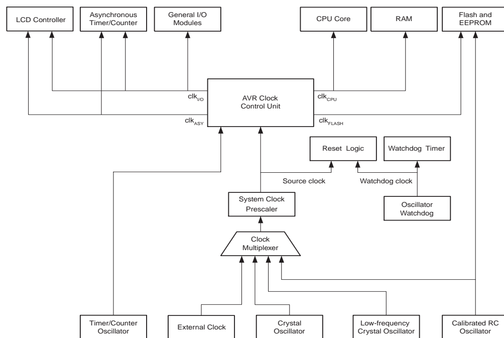
Figure 11. Clock Distribution
