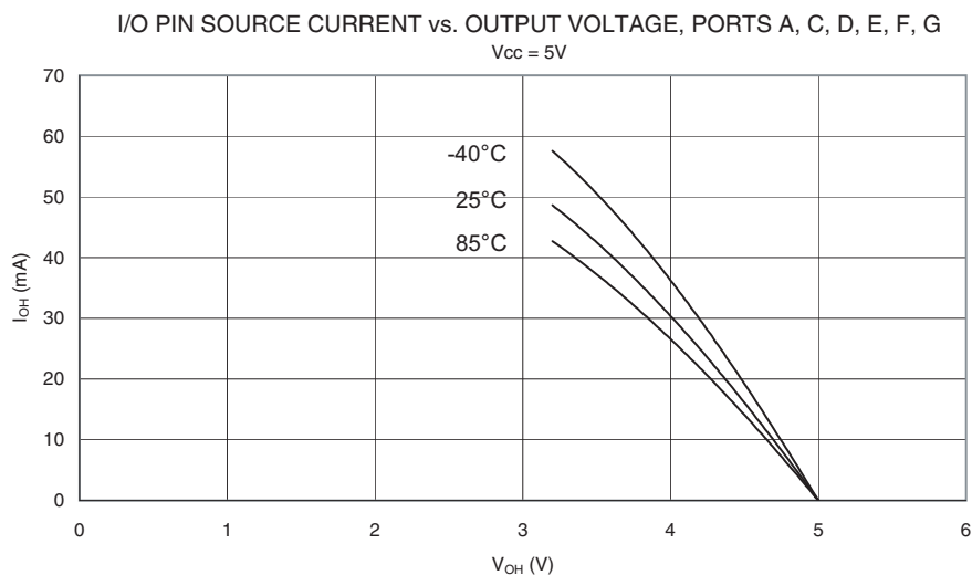
Figure 168. I/O Pin Source Current vs. Output Voltage, Ports A, C, D, E, F, G ( V_{CC} = 2.7V )
