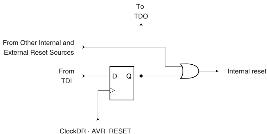
Figure 108. Reset Register
