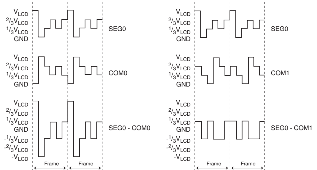
Figure 101. Driving a LCD with Three Common Terminals
