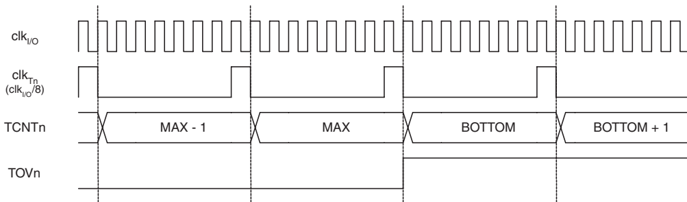
Figure 35. Timer/Counter Timing Diagram, with Prescaler ( f_{\text{clk\_I/O}}/8 )
