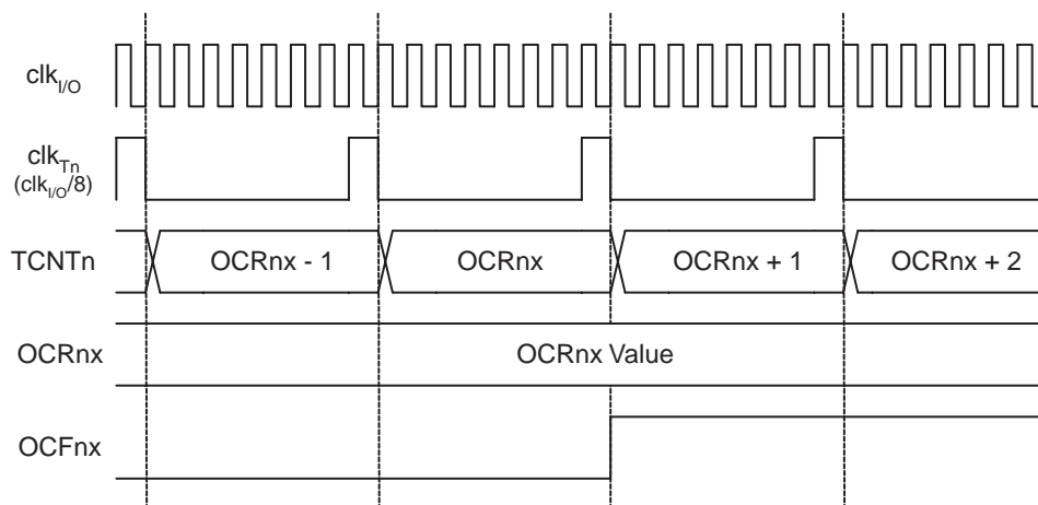
Figure 62. Timer/Counter Timing Diagram, Setting of OCF2A, with Prescaler ( f_{clk\_I/O}/8 )
