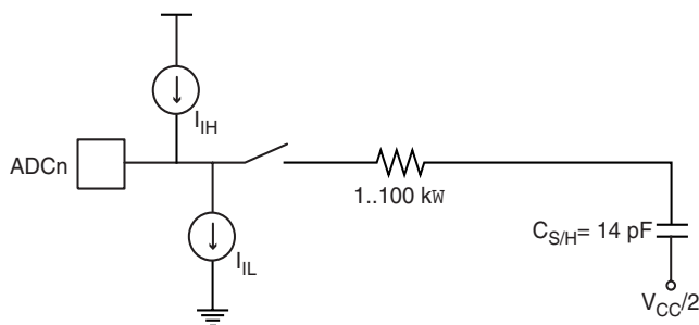
Figure 90. Analog Input Circuitry
