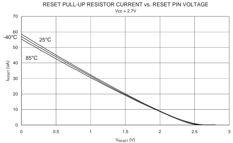
Figure 165. Reset Pull-up Resistor Current vs. Reset Pin Voltage ( V_{CC} = 2.7V )
