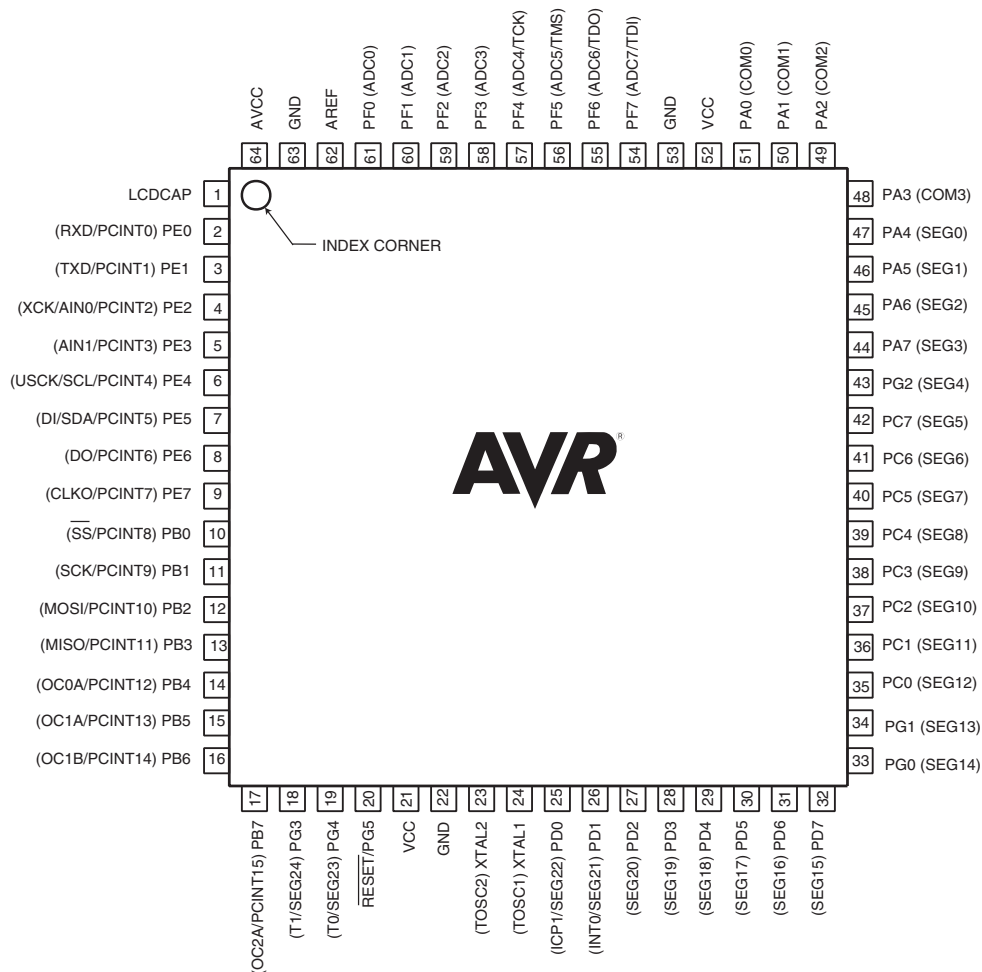
Figure 1-1. Pinout ATmega169P
