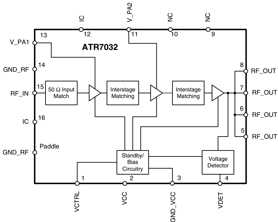
Figure 1-1. Block Diagram
