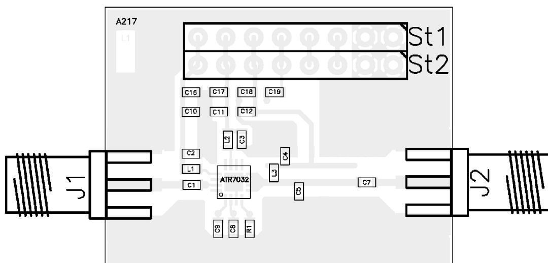
Figure 10-2. Application Board Layout
