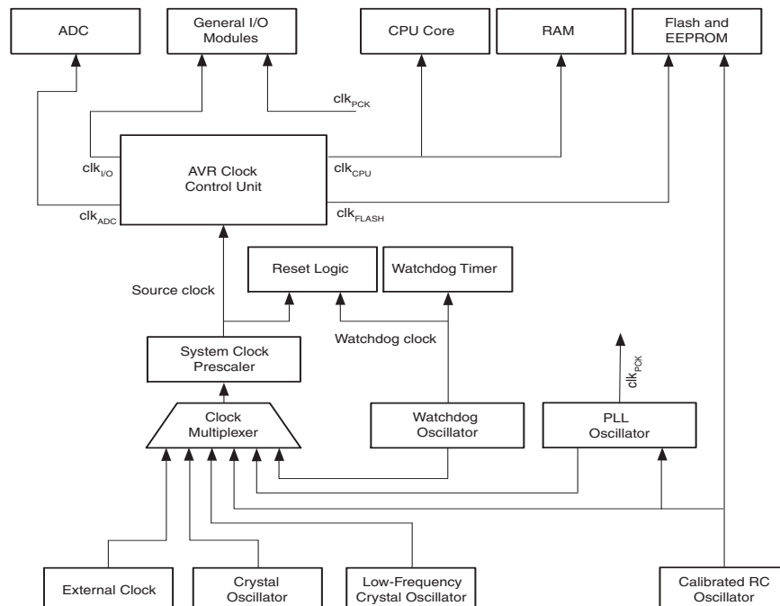
Figure 6-1. Clock Distribution
