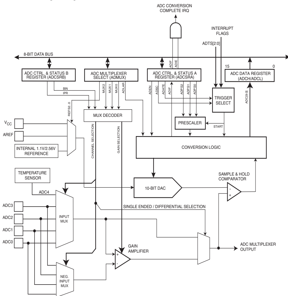
Figure 19-1. Analog to Digital Converter Block Schematic
