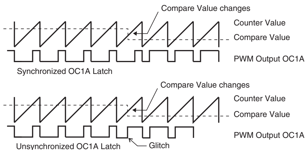
Figure 15-4. Effects of Unsynchronized OCR Latching
