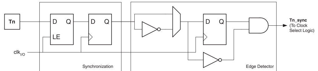
Figure 13-1. T0 Pin Sampling
