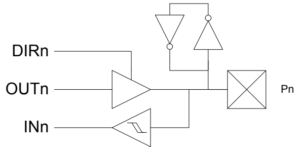
Figure 14-4. I/O configuration - Totem-pole with bus-keeper
