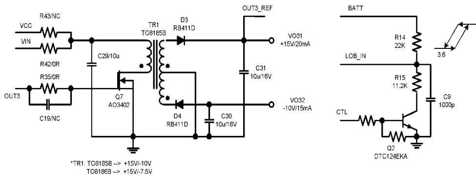
POWER CH3(FLYBACK)
