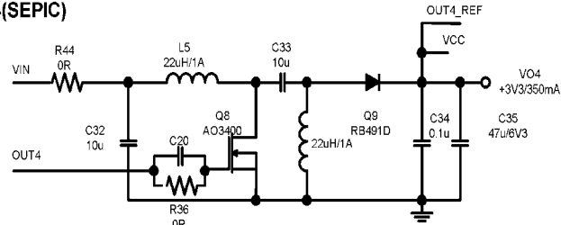
POWER CH1(STEP-DOWN)
