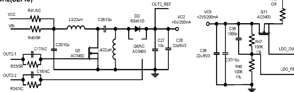
POWER CH2(SEPIC)
