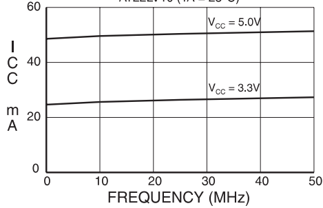
SUPPLY CURRENT vs. INPUT FREQUENCY AT22LV10 (TA = 25°C)
