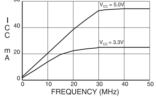
SUPPLY CURRENT vs. INPUT FREQUENCY AT22LV10L (TA = 25°C)
