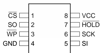
8-Pin SOIC
