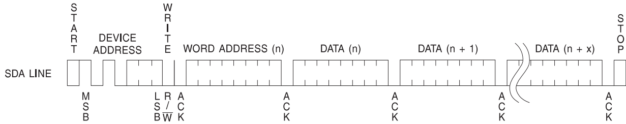
Figure 12. Page Write
