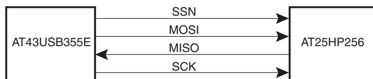
Figure 4. AT43USB355E Read Sequence
