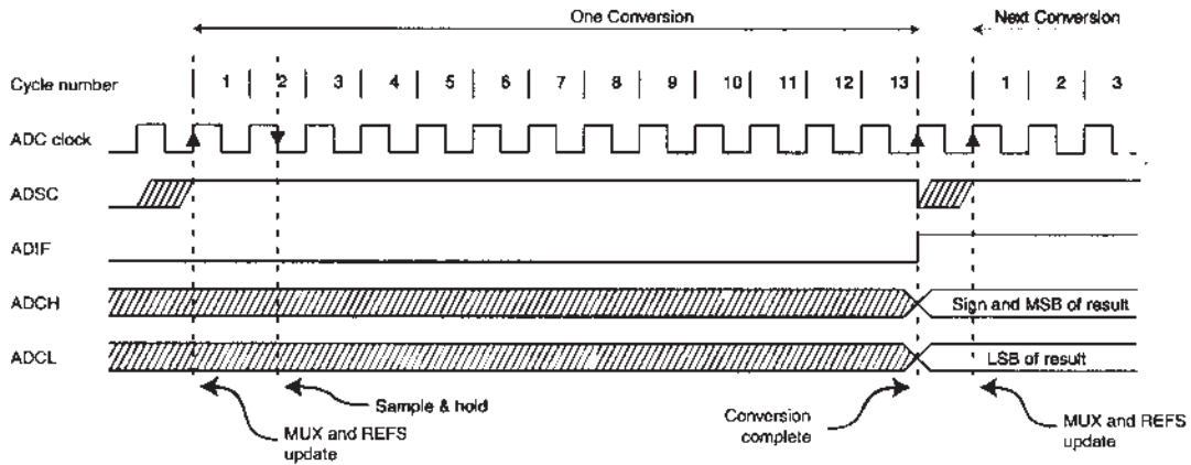
Figure 25. ADC Timing Diagram, Single Conversion
