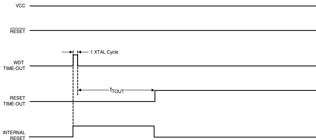
Figure 11. Watchdog Reset During Operation
