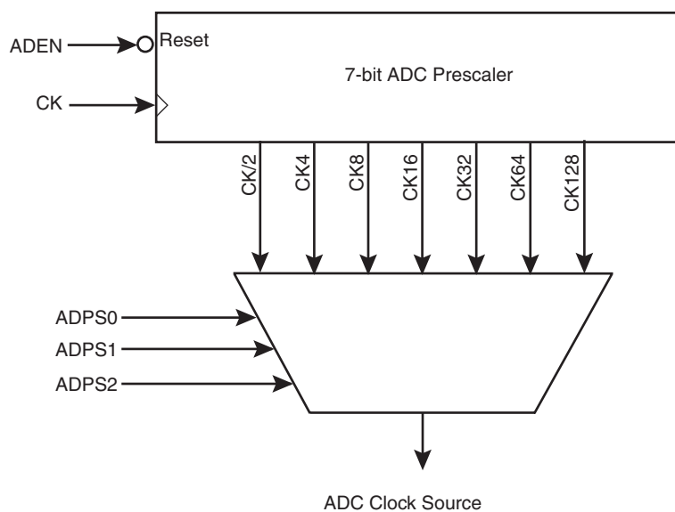
Figure 23. ADC Prescaler
