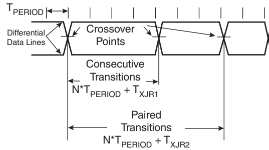
Figure 31. Differential Data Jitter
