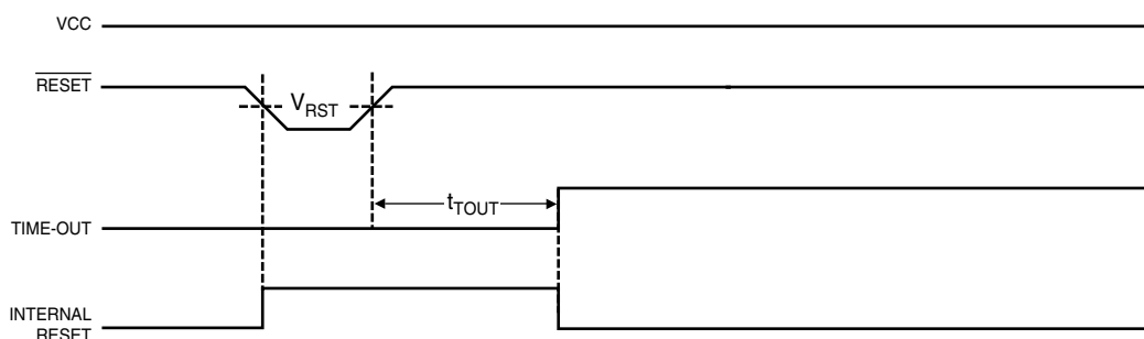
Figure 10. External Reset During Operation
