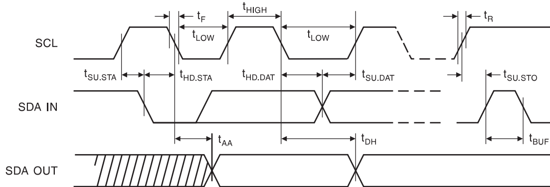
Figure 3. Bus Timing for 2 wire communications SCL: Serial Clock, SDA: Serial Data I/O
