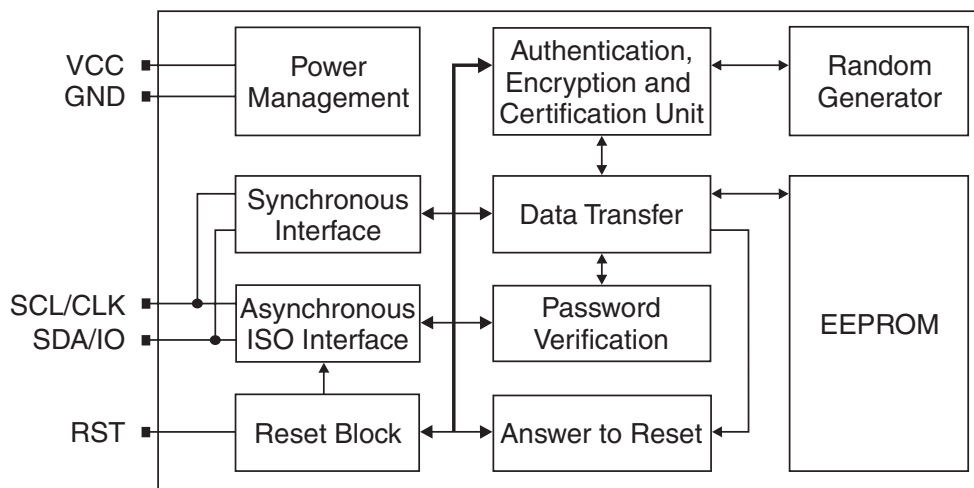
Figure 2. Block Diagram
