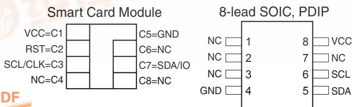
Figure 1. Package Options
