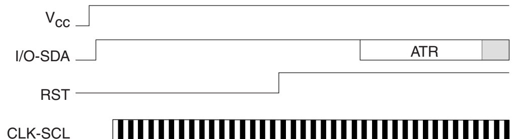
Figure 10. Asynchronous T = 0 Protocol (Gemplus Patent)
