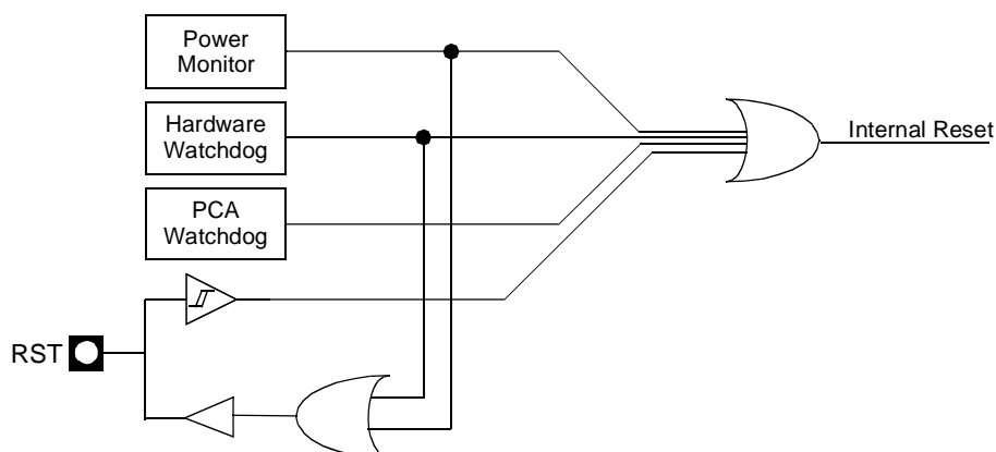
Figure 71. Reset schematic
