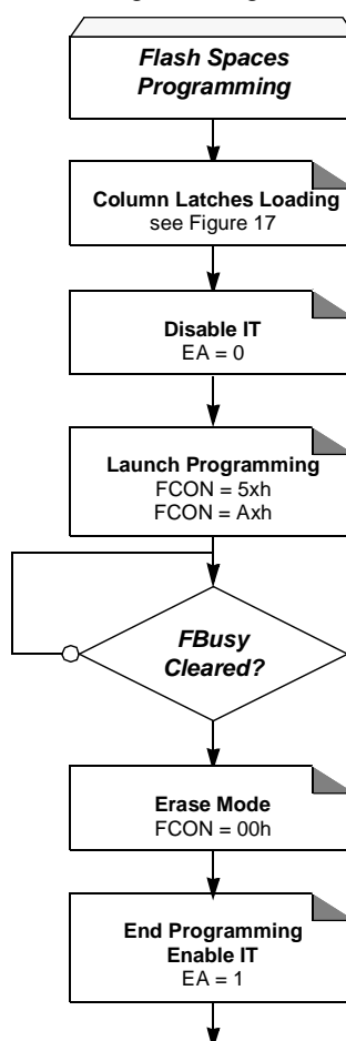
Figure 18. Flash and Extra Row Programming Procedure
