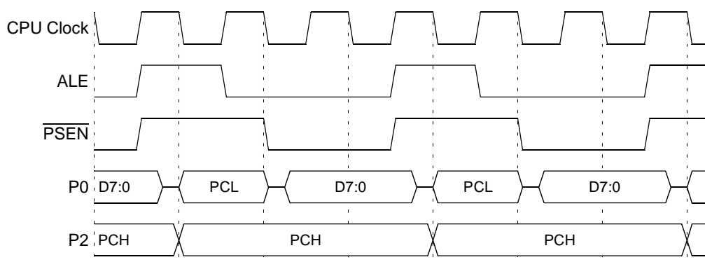
Figure 15. External Code Fetch Waveforms
