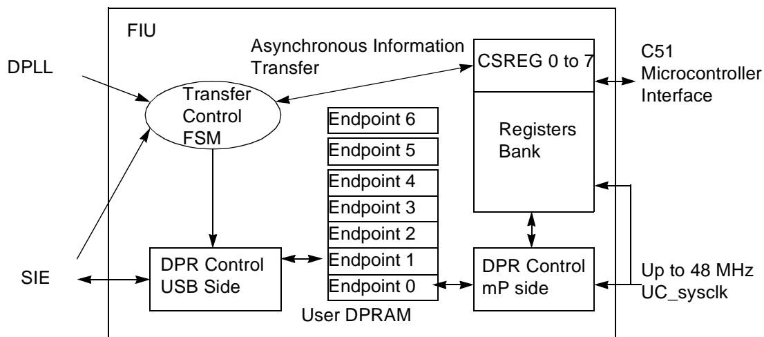
Figure 57. UFI Block Diagram
