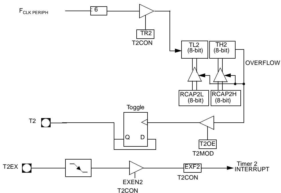
Figure 26. Clock-out Mode C/\overline{T2} = 0
