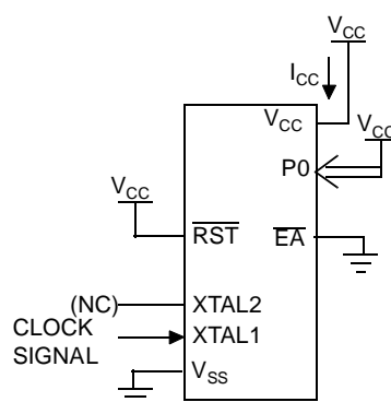
Figure 78. I_{CC} Test Condition, Idle Mode
