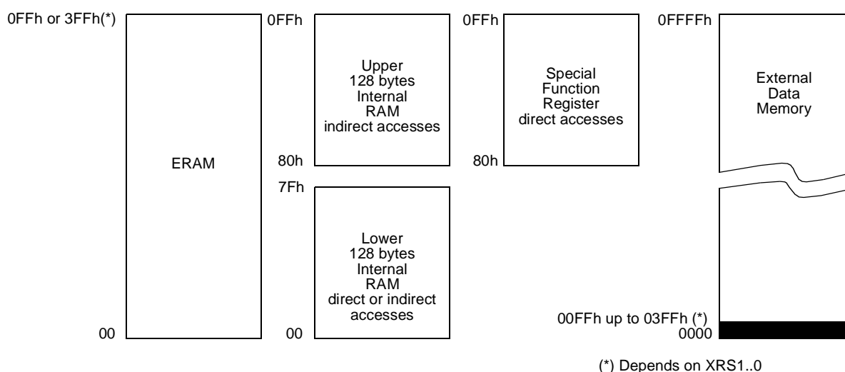
Figure 24. Internal and External Data Memory Address
