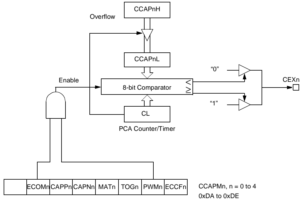
Figure 32. PCA PWM Mode
