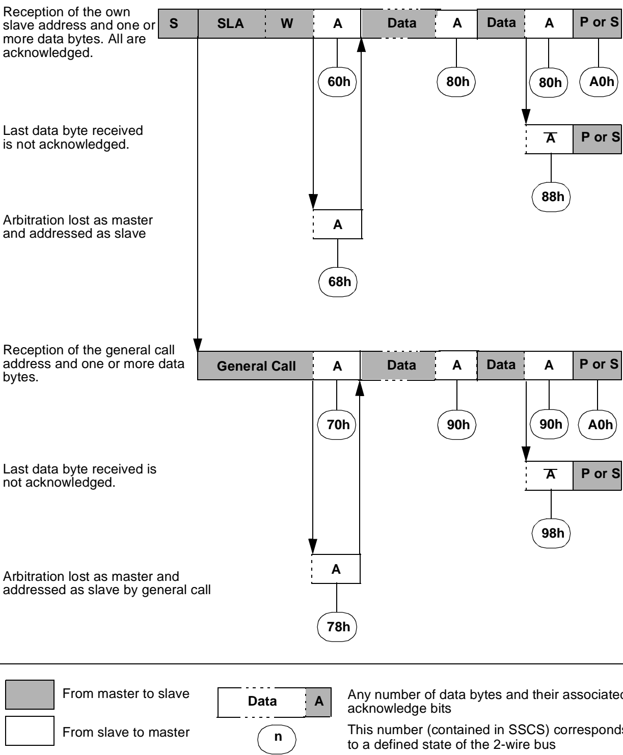
Figure 53. Format and State in the Slave Receiver Mode
