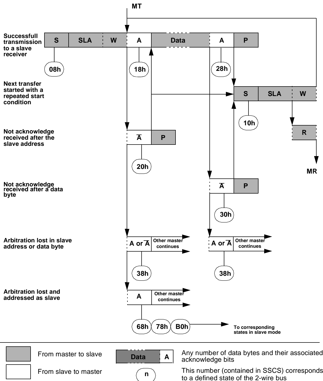
Figure 51. Format and State in the Master Transmitter Mode
