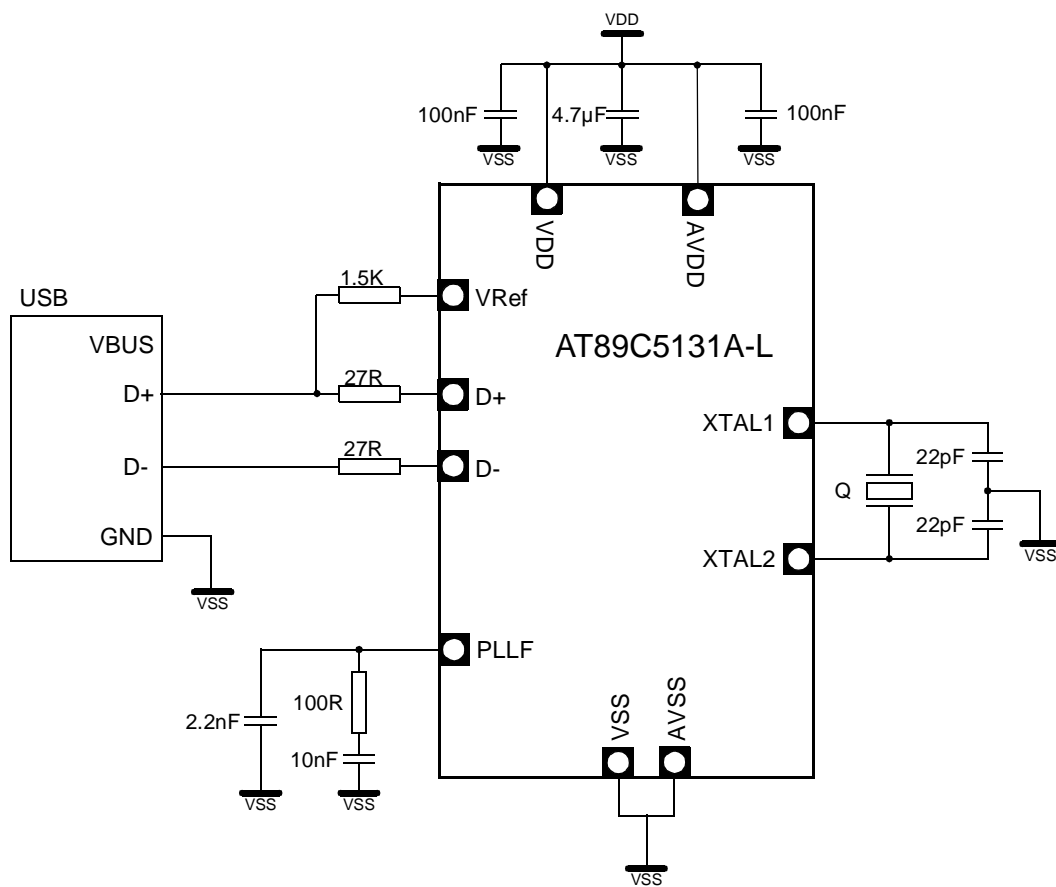
Figure 4. Typical Application
