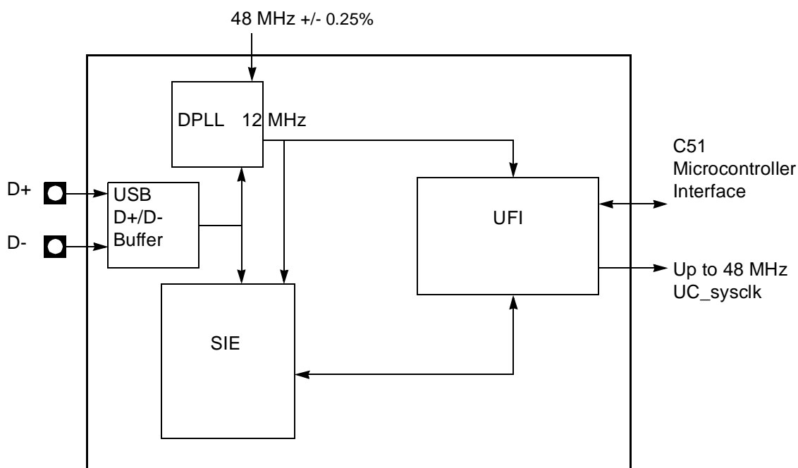
Figure 55. USB Device Controller Block Diagram
