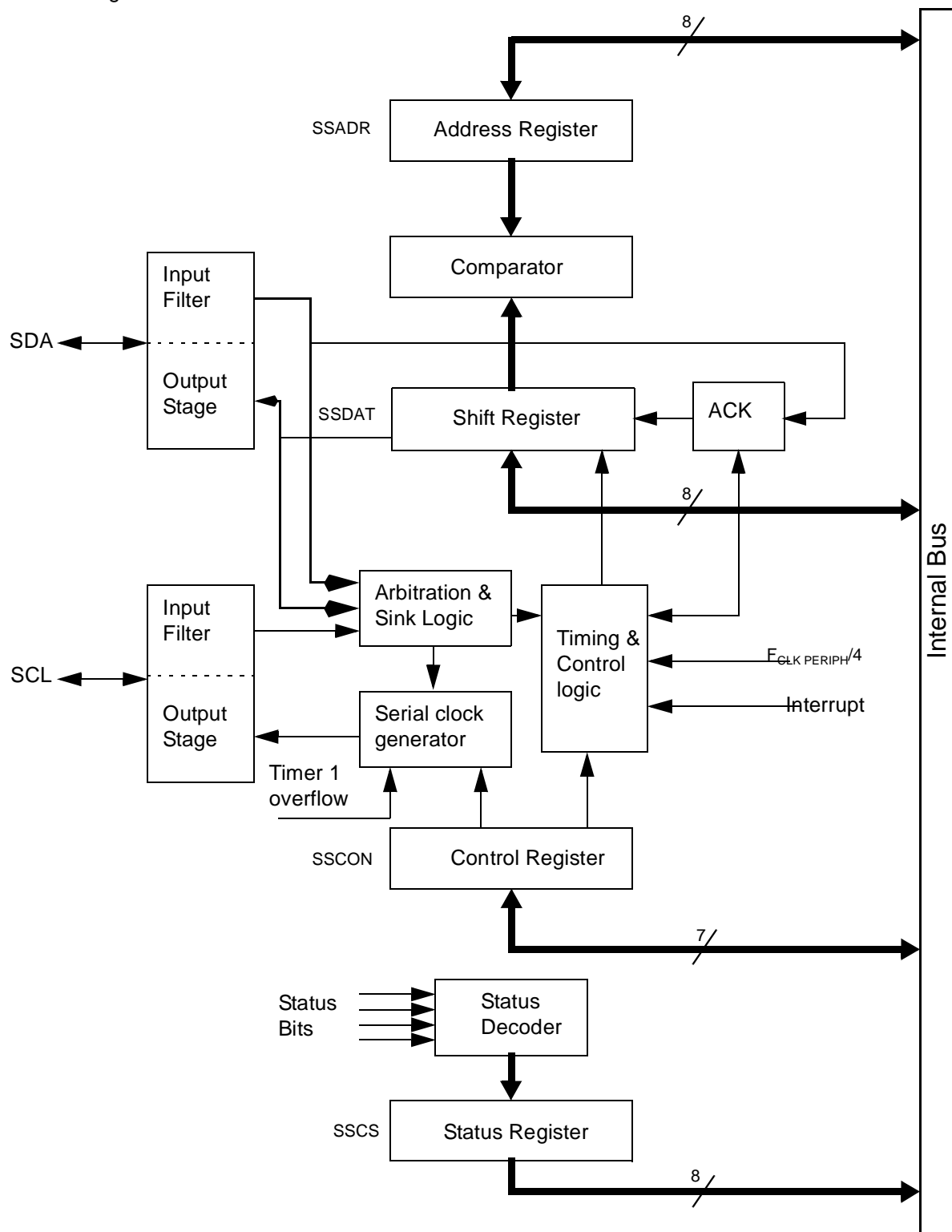
Figure 49. Block Diagram
