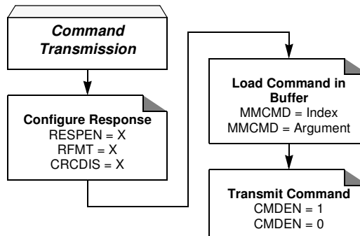
Figure 16-13. Command Transmission Flow
