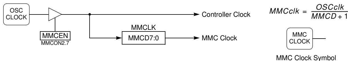
Figure 16-10. MMC Clock Generator and Symbol
