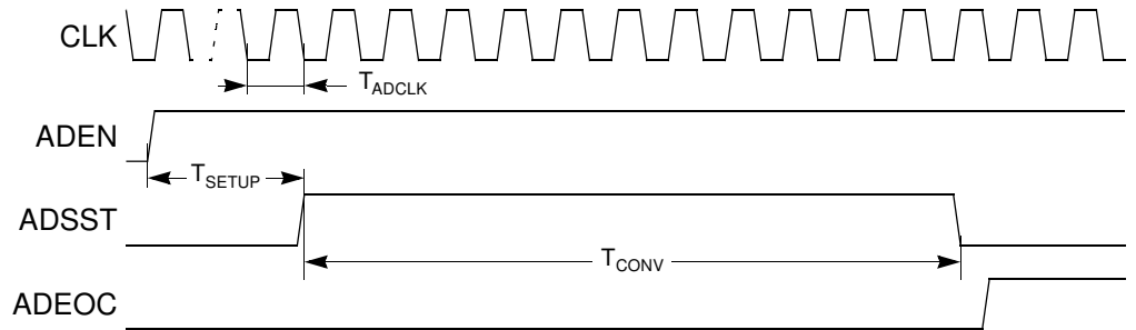
Figure 21-2. Timing Diagram
