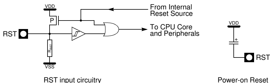
Figure 11-1. Reset Circuitry and Power-On Reset
