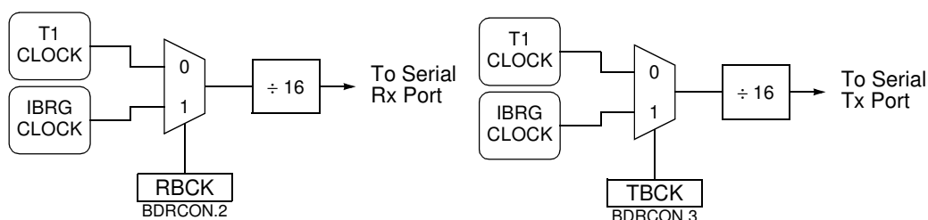
Figure 18-12. Baud Rate Source Selection (Modes 1 and 3)
