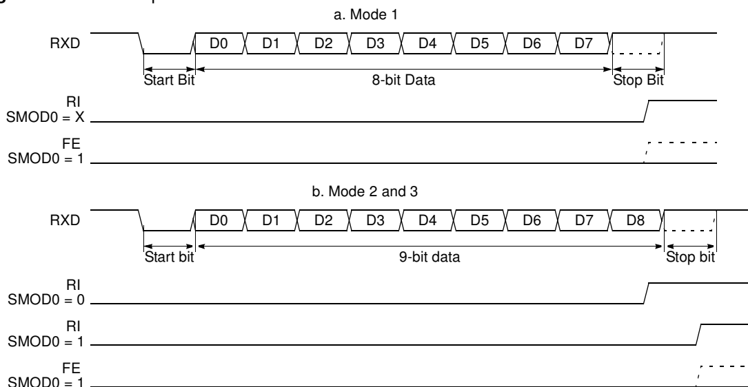
Figure 18-17. Interrupt Waveforms
