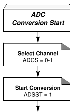
Figure 21-5. ADC Conversion Launching Flow
