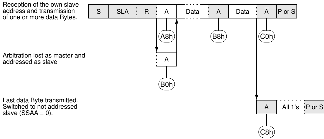
Figure 20-6. Format and States in the Slave Transmitter Mode
