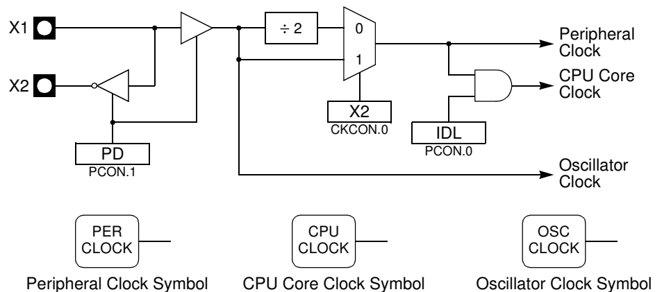
Figure 6-2. Crystal Connection
