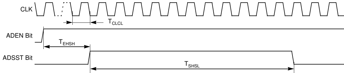
Figure 23-19. Analog-to-Digital Converter Internal Waveforms
