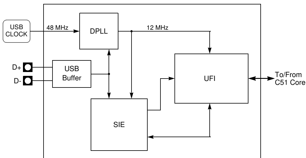
Figure 15-1. USB Device Controller Block Diagram
