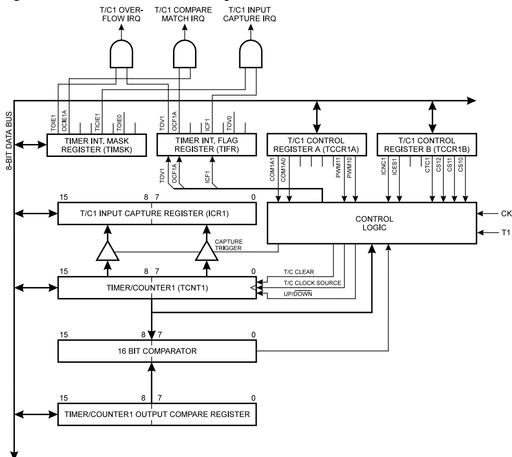
Figure 30 shows the block diagram for Timer/Counter1.
