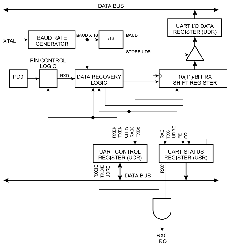
Figure 35. UART Receiver
