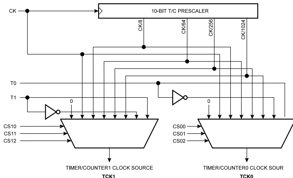
Figure 28. Timer/Counter Prescaler
