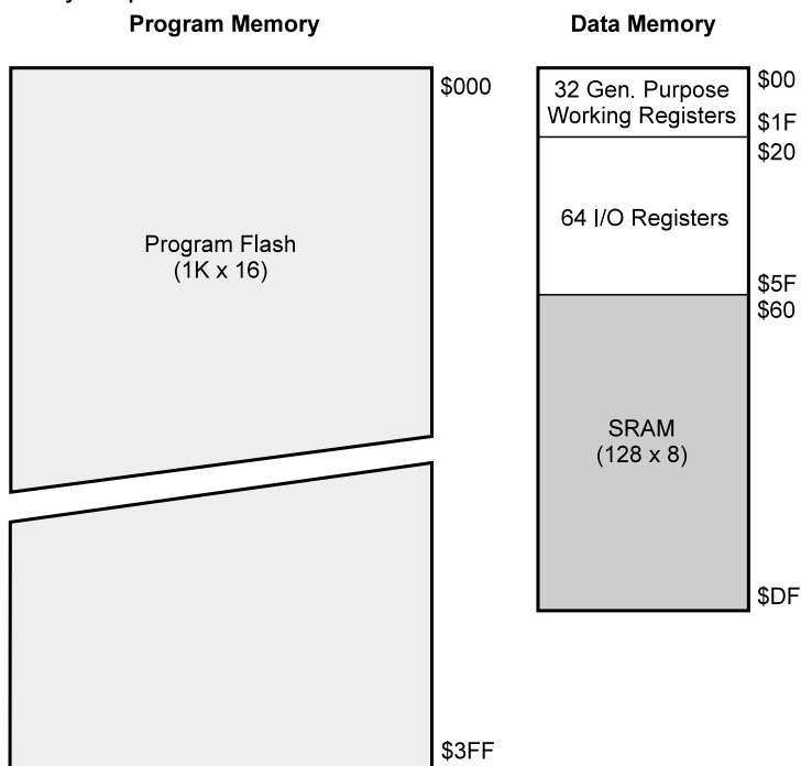
Figure 5. Memory Maps
