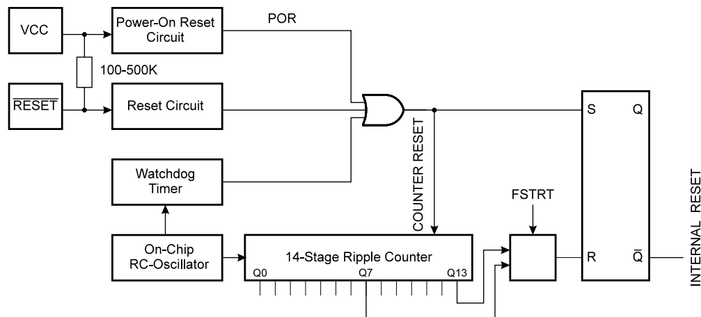
Figure 23. Reset Logic
