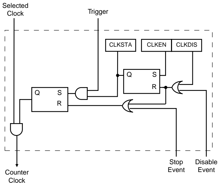
Figure 43. Clock Control
