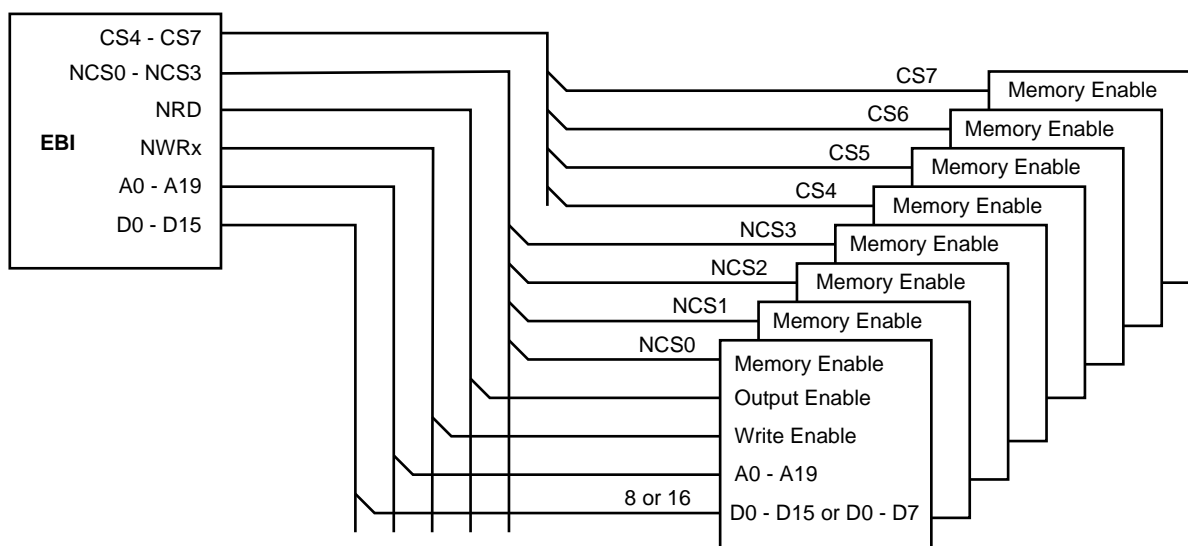
Figure 7. Memory Connections for Eight External Devices
