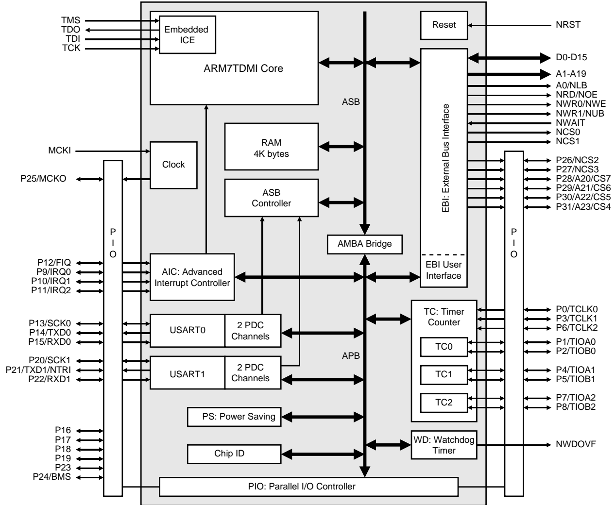
Figure 2. AT91M40400
