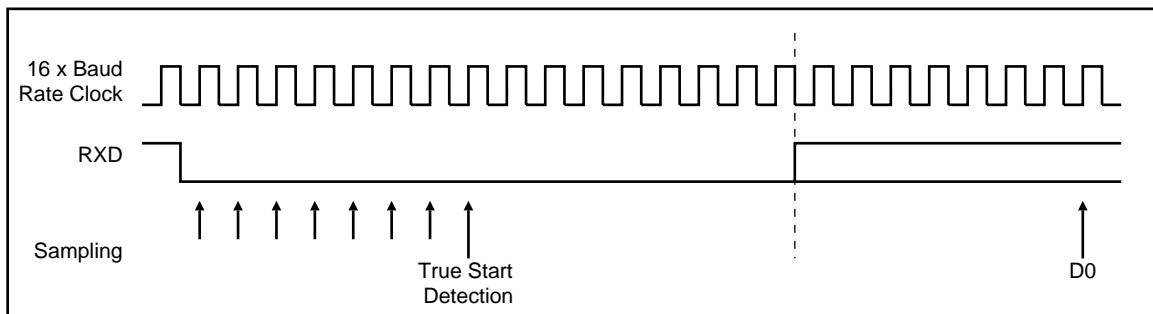
Figure 36. Asynchronous Mode: Start Bit Detection
