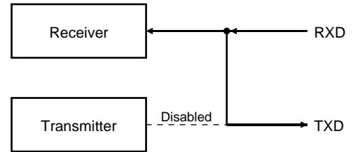
Figure 40. Channel Modes
