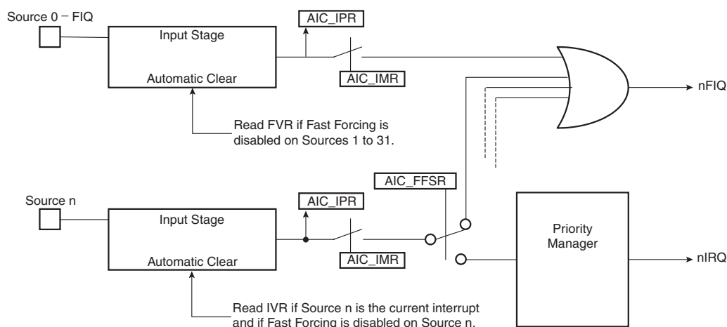
Figure 22-10. Fast Forcing
