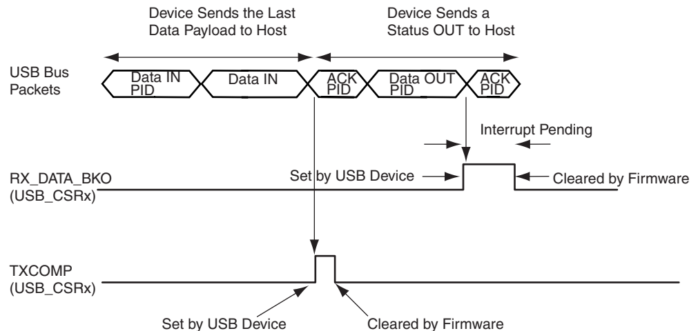
Figure 33-14. Data IN Followed by Status OUT Transfer
