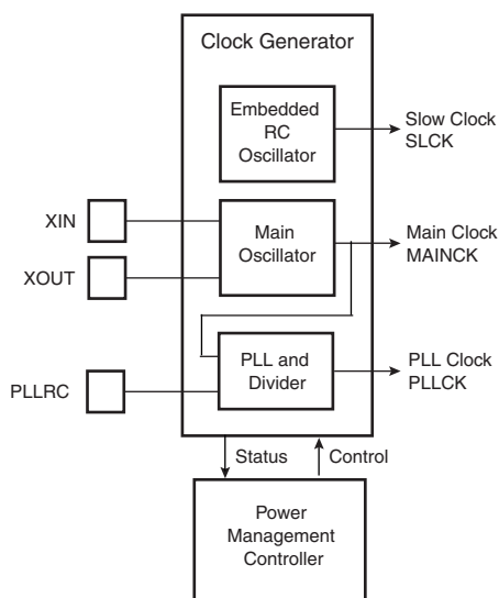
Figure 9-3. Clock Generator Block Diagram
