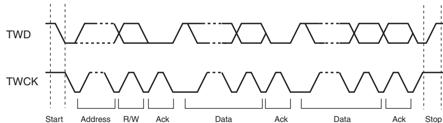
Figure 28-4. Transfer Format
