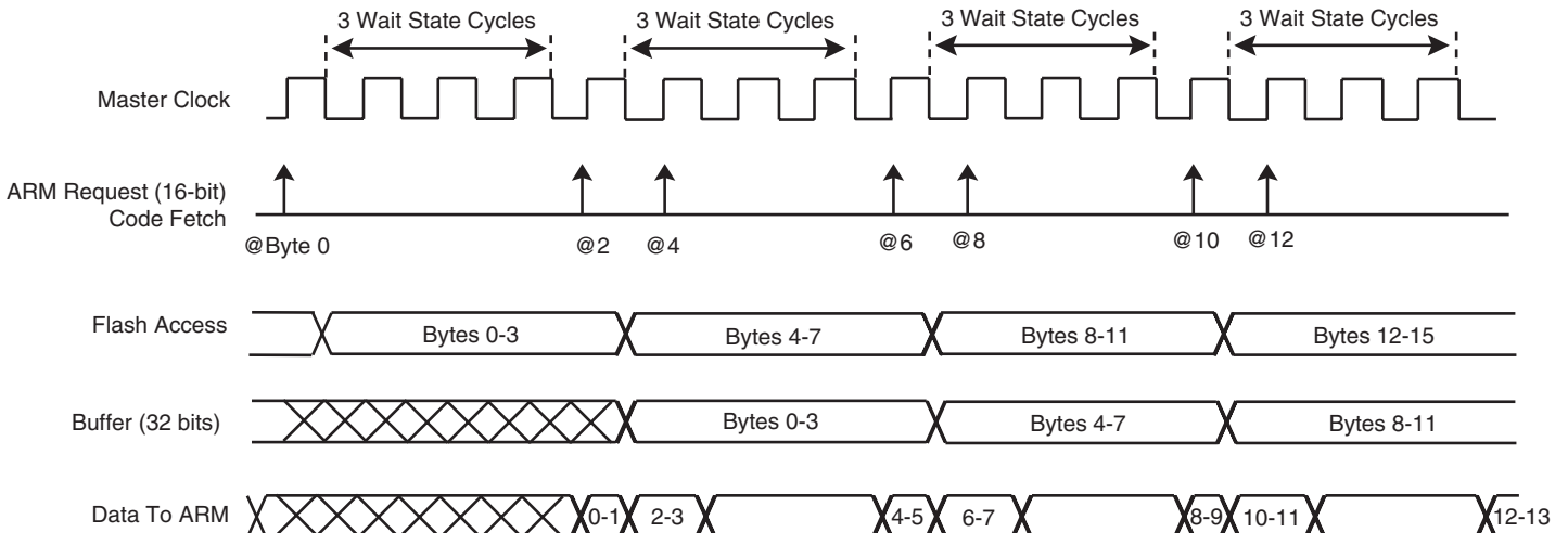
Figure 19-4. Code Read Optimization in Thumb Mode for FWS = 3
