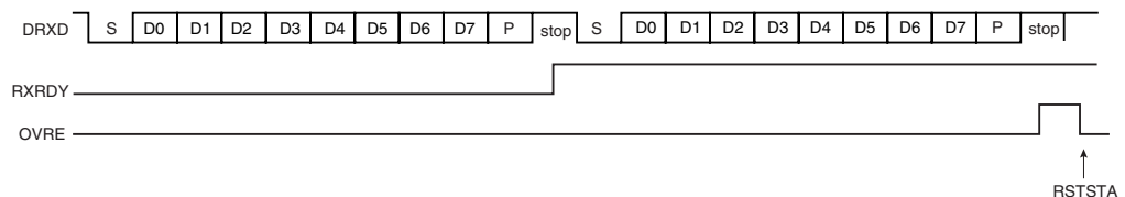
Figure 25-7. Receiver Overrun
