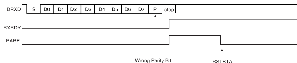
Figure 25-8. Parity Error
