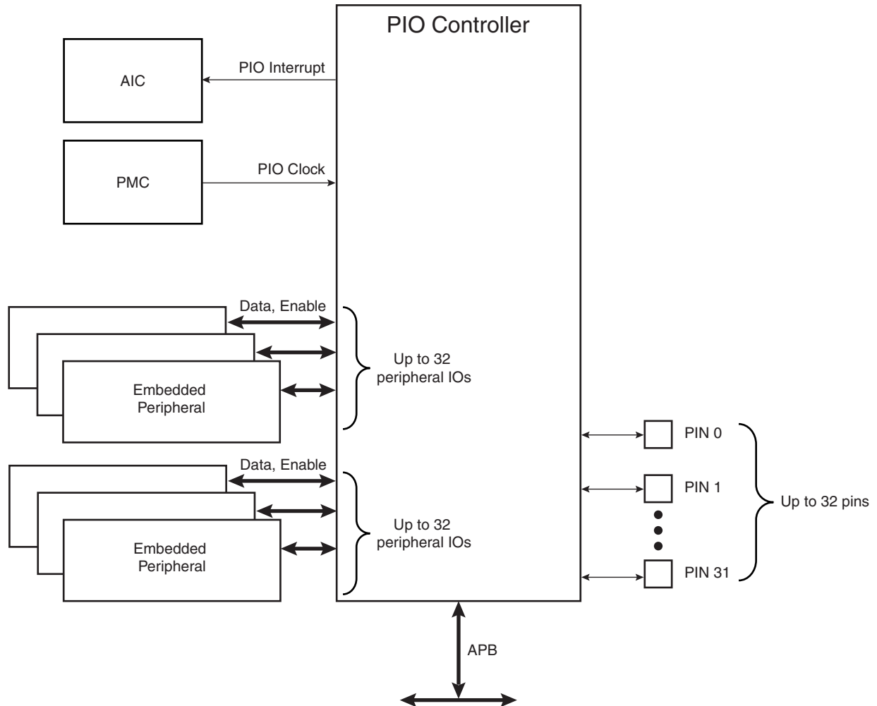
Figure 26-1. Block Diagram
