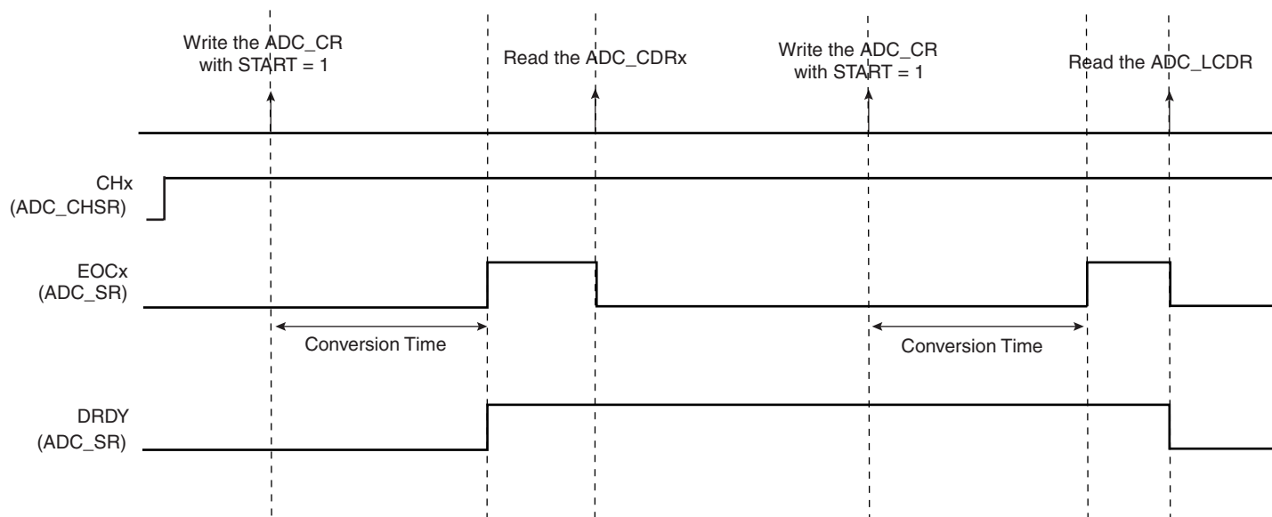
Figure 34-2. EOCx and DRDY Flag Behavior
