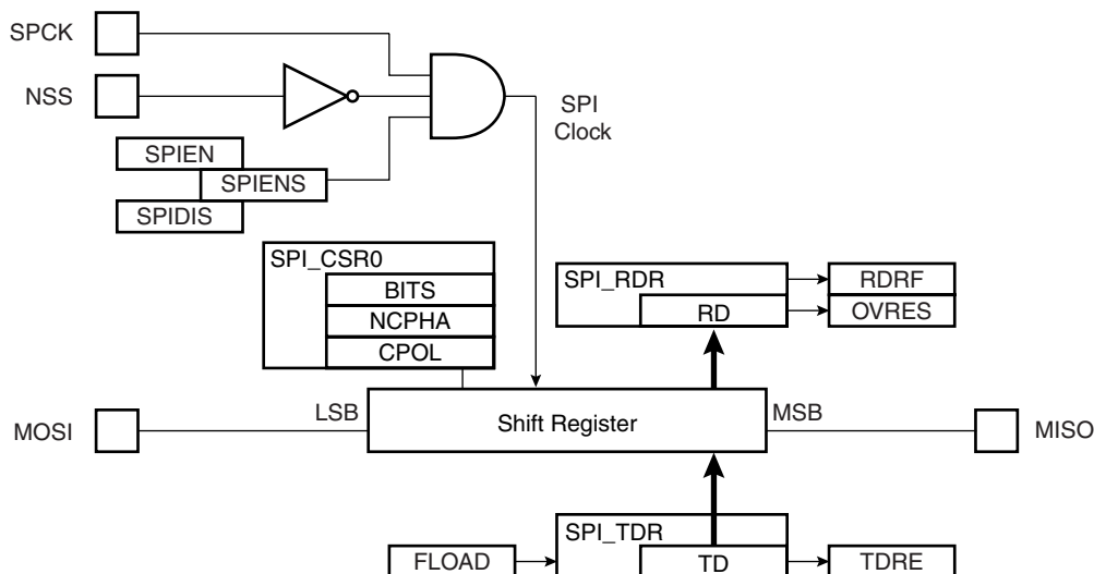
Figure 27-9. Slave Mode Functional Block Diagram
