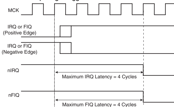
Figure 22-6. External Interrupt Edge Triggerged Source
