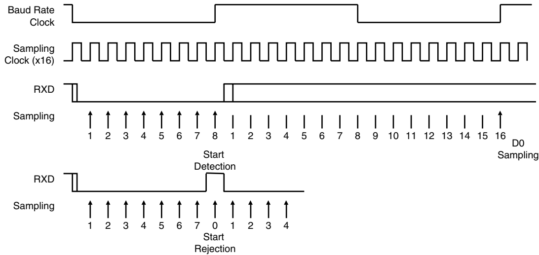
Figure 29-8. Asynchronous Character Reception
