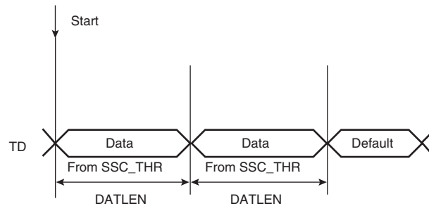
Figure 30-13. Transmit Frame Format in Continuous Mode
