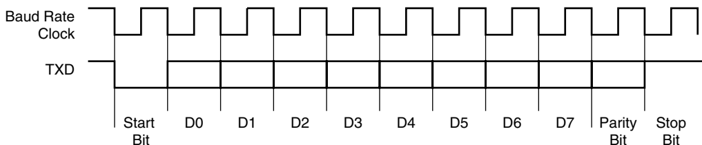
Figure 29-5. Character Transmit
