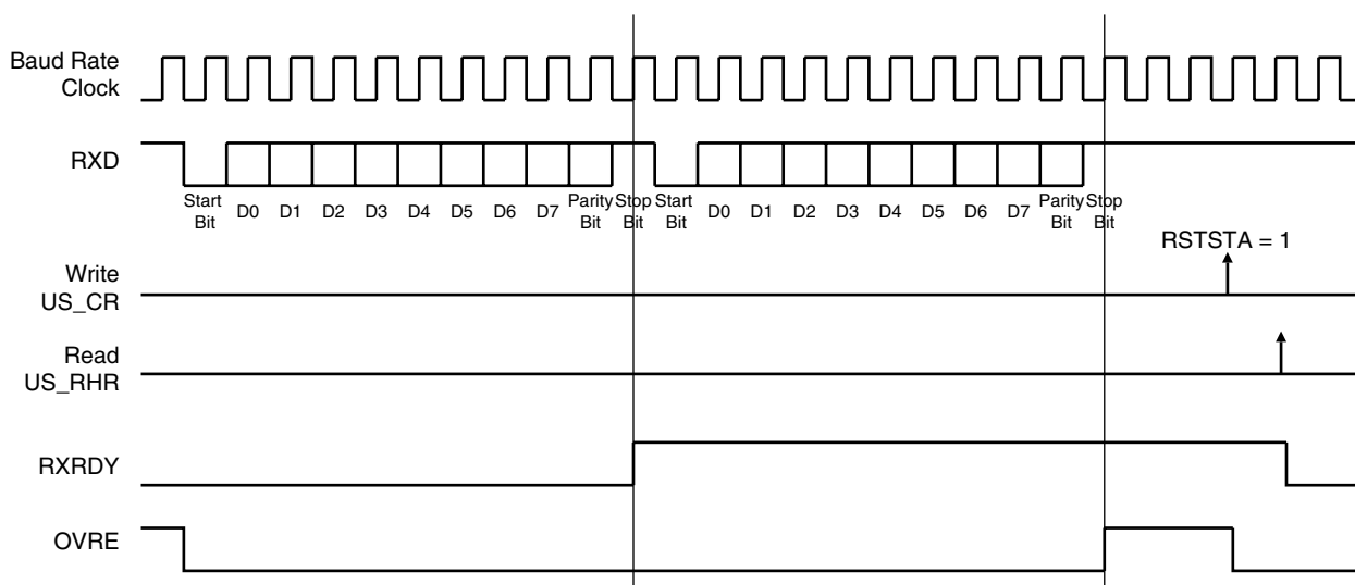
Figure 29-10. Receiver Status
