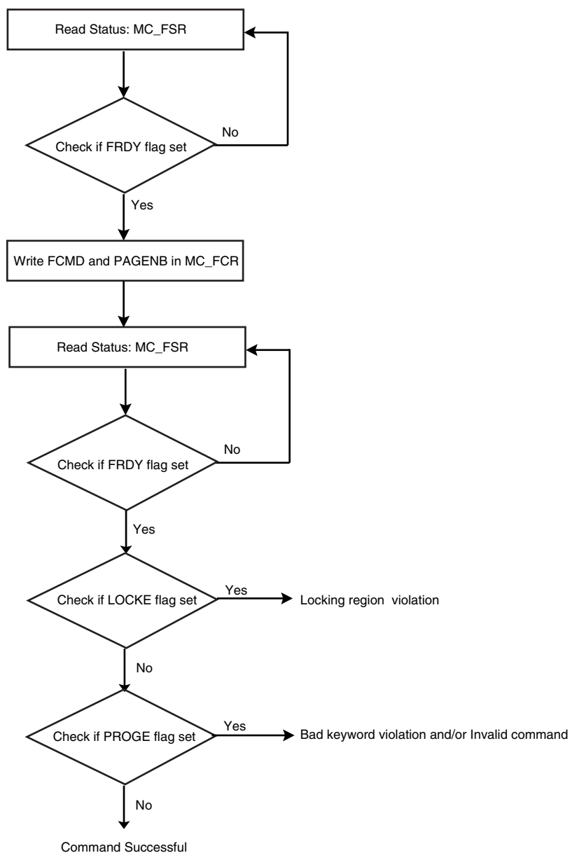
Figure 19-5. Command Statechart
