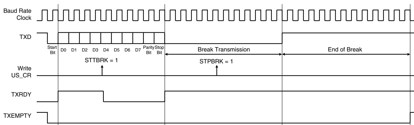
Figure 29-15. Break Transmission
