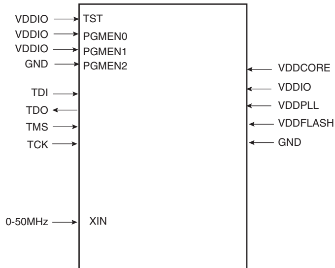
Figure 20-4. Serial Programming
