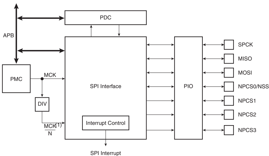
Figure 27-1. Block Diagram
