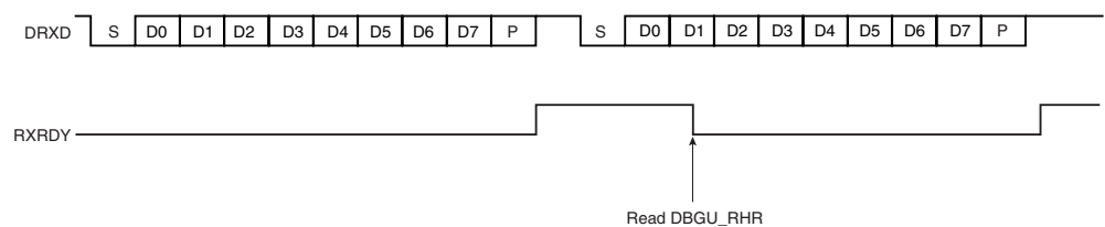
Figure 25-6. Receiver Ready
