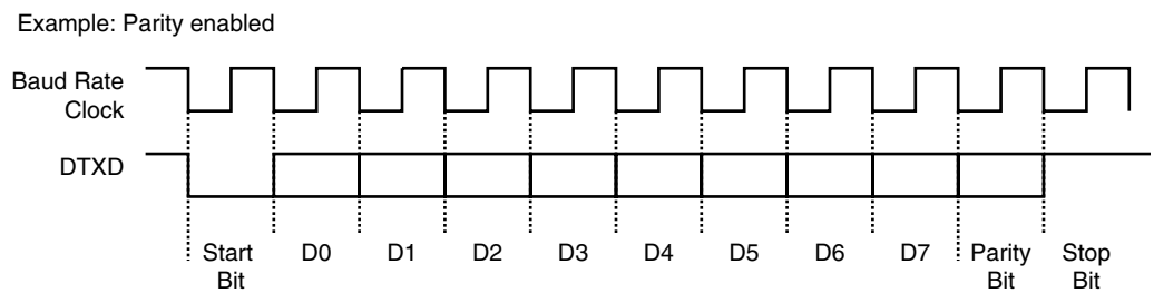
Figure 25-10. Character Transmission
