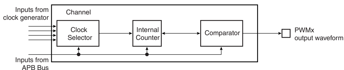
Figure 32-3. Functional View of the Channel Block Diagram
