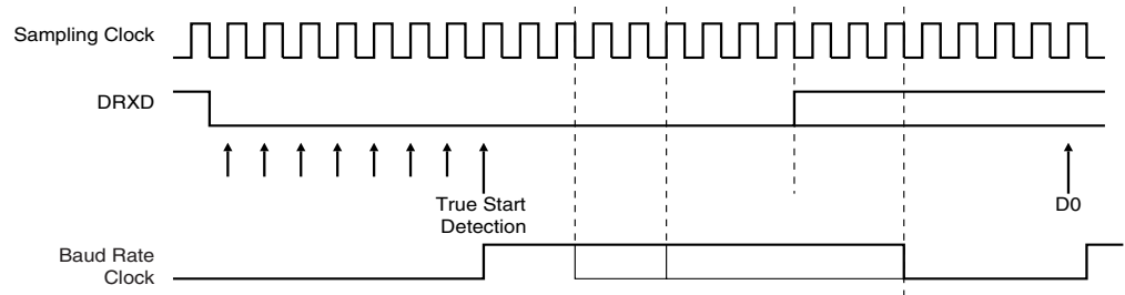
Figure 25-4. Start Bit Detection
