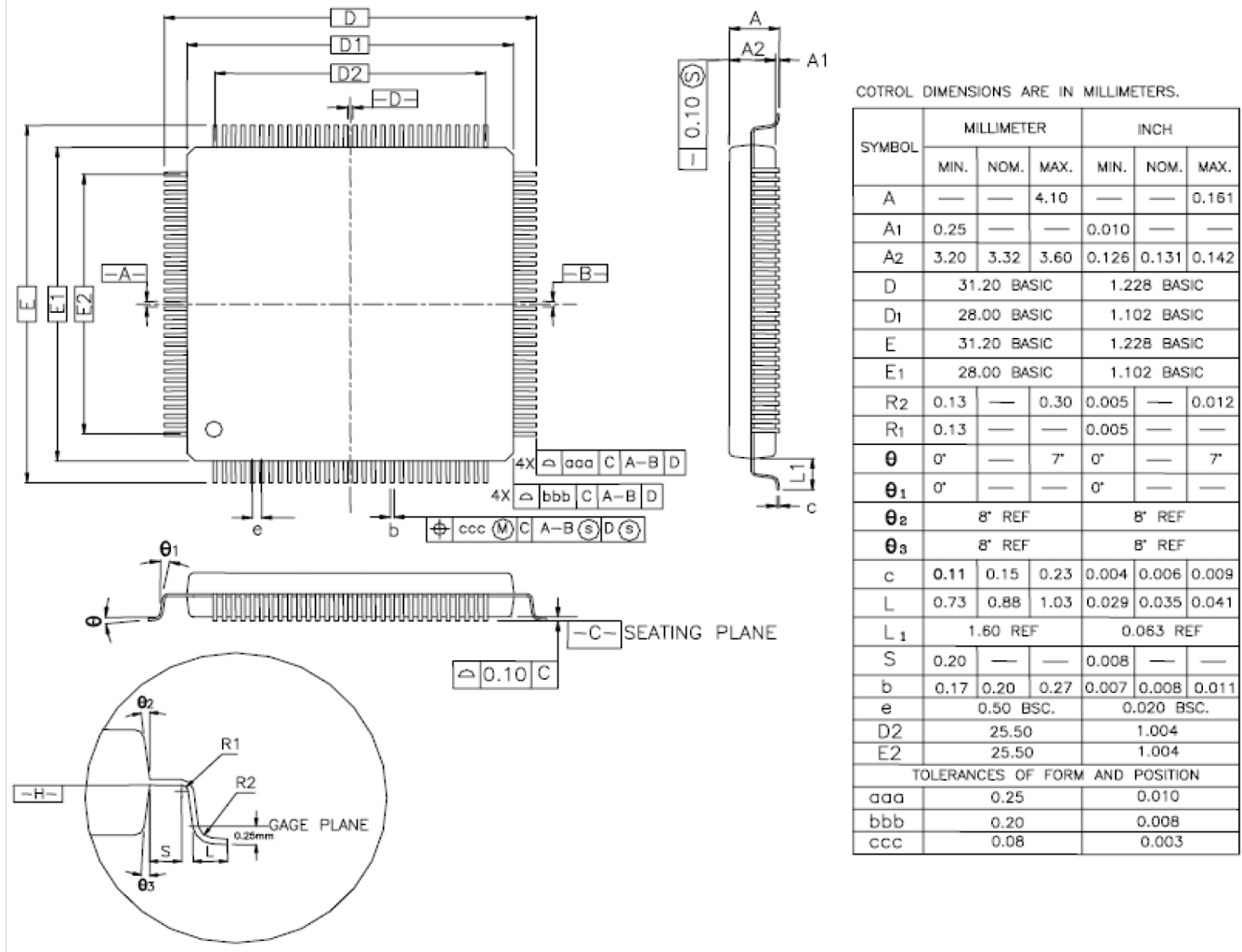
Figure 11-1. 208-lead TQFP Package Drawing
