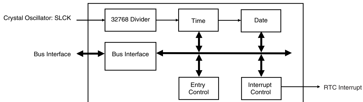
Figure 20-1. Block Diagram
