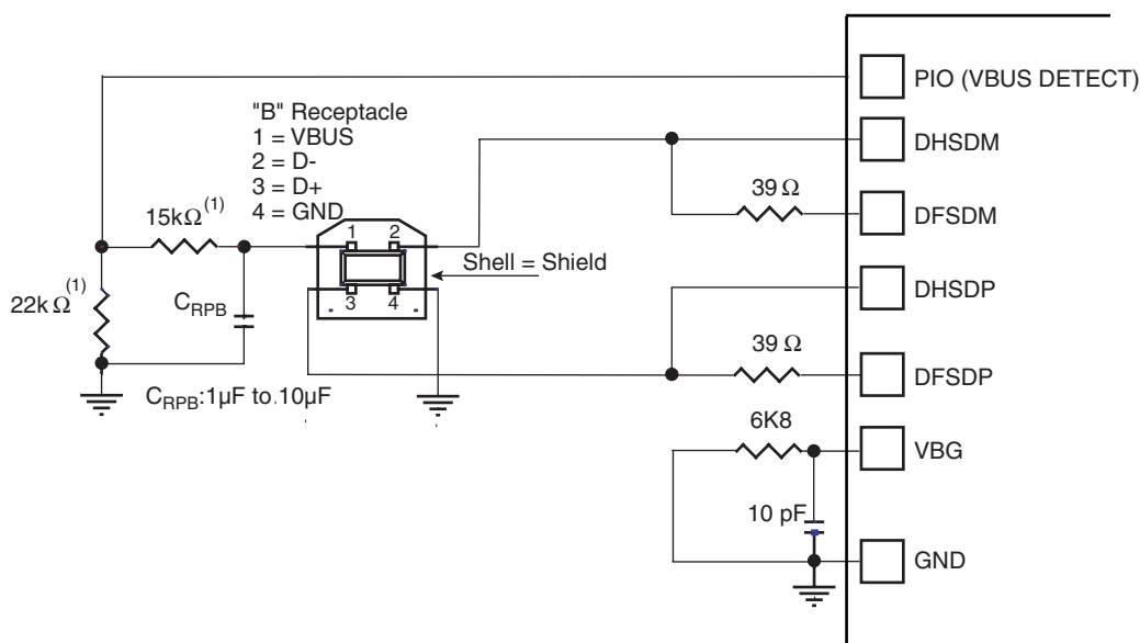
Figure 41-2. Board Schematic
