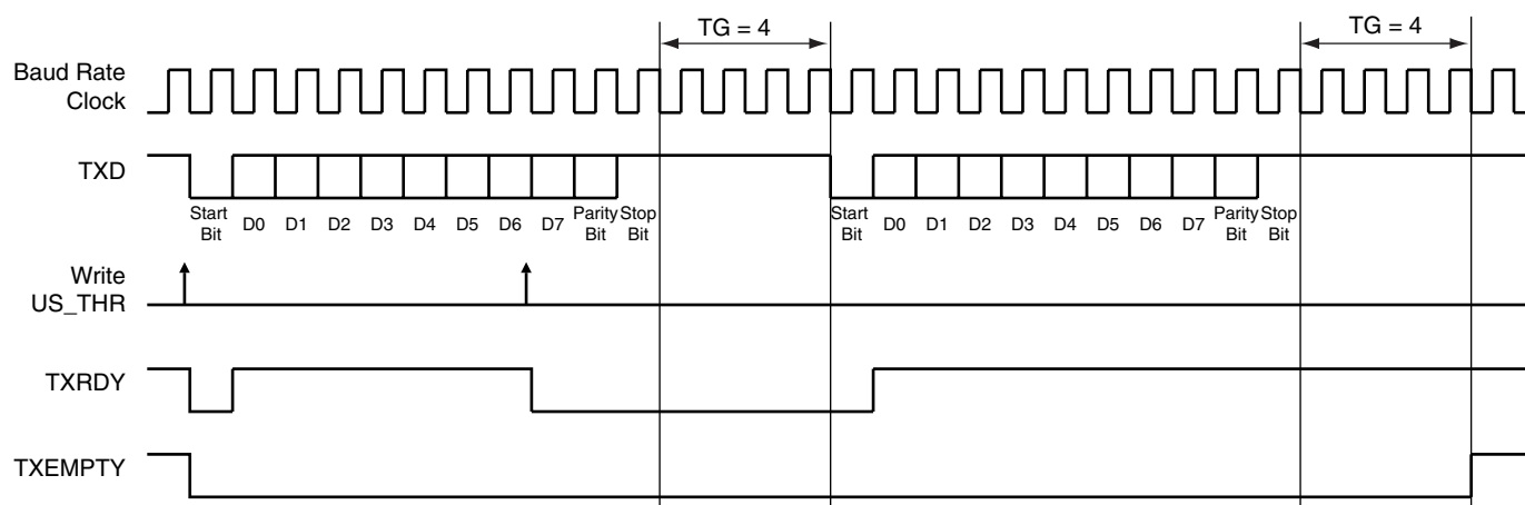
Figure 34-23. Timeguard Operations
