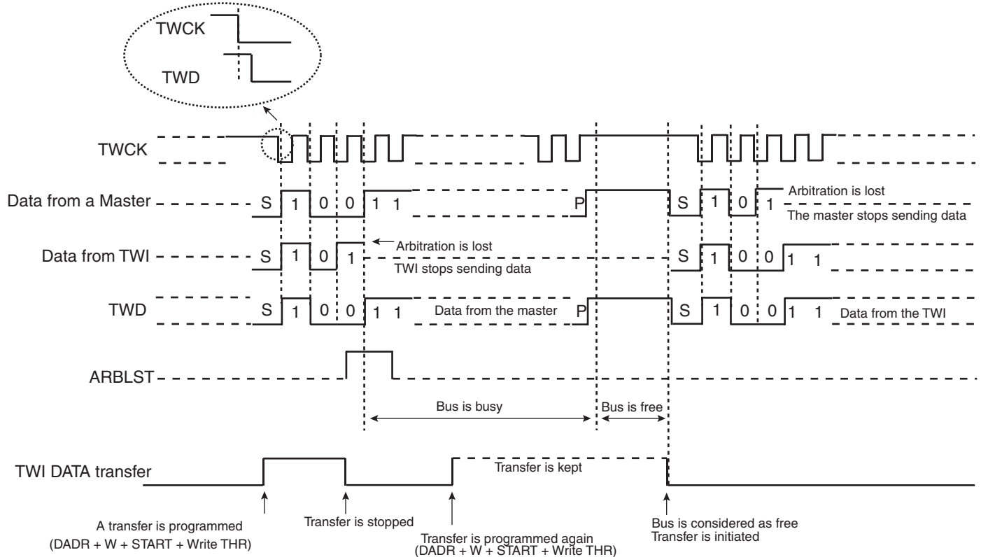
Figure 33-21. Arbitration Cases
