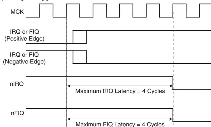
Figure 29-6. External Interrupt Edge Triggered Source
