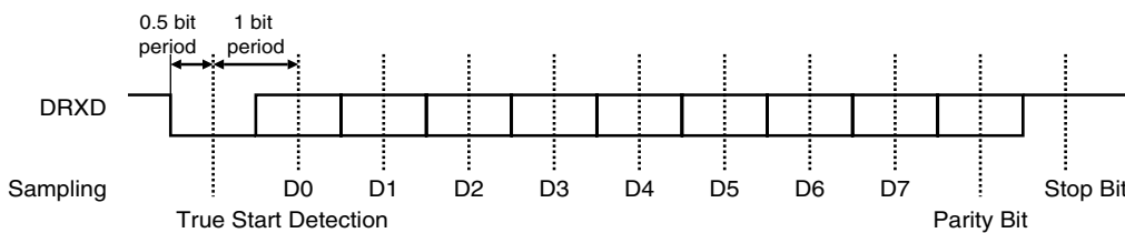
Figure 30-5. Character Reception
