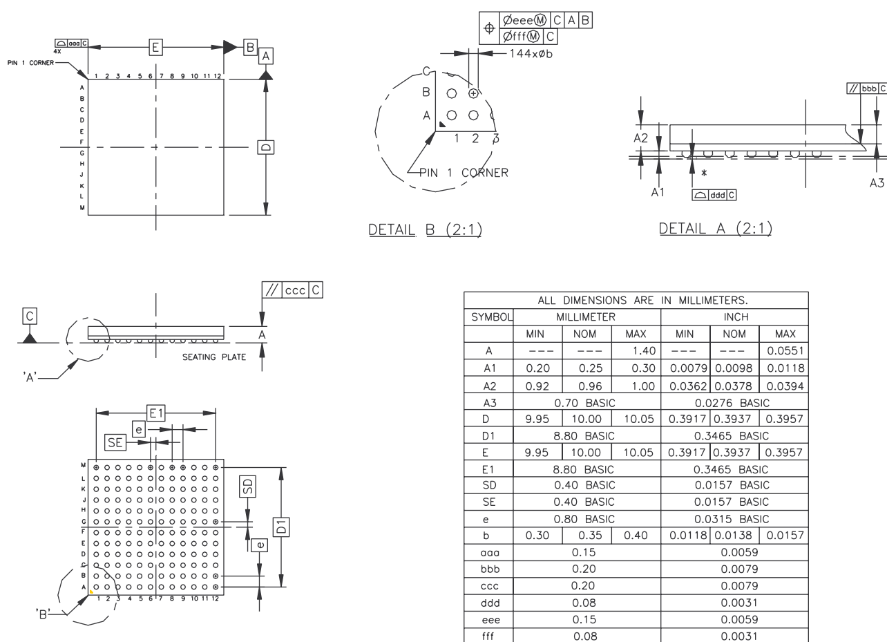
Figure 45-1. 144-ball BGA Package Drawing
