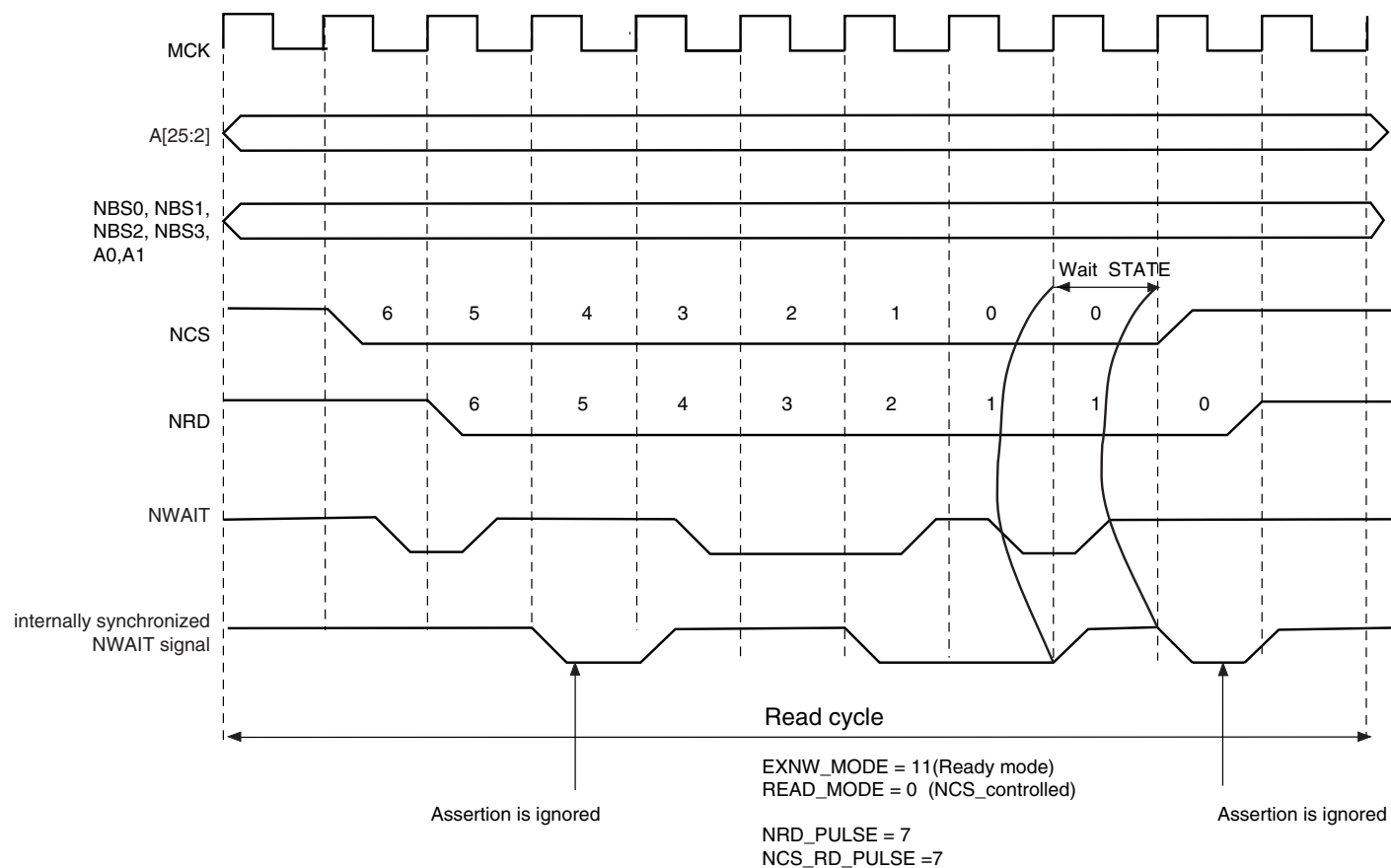
Figure 23-29. NWAIT Assertion in Read Access: Ready Mode (EXNW_MODE = 11)
