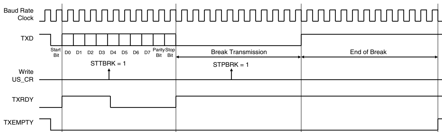
Figure 34-26. Break Transmission
