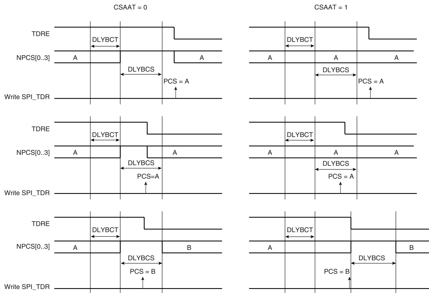
Figure 32-8. Peripheral Deselection
