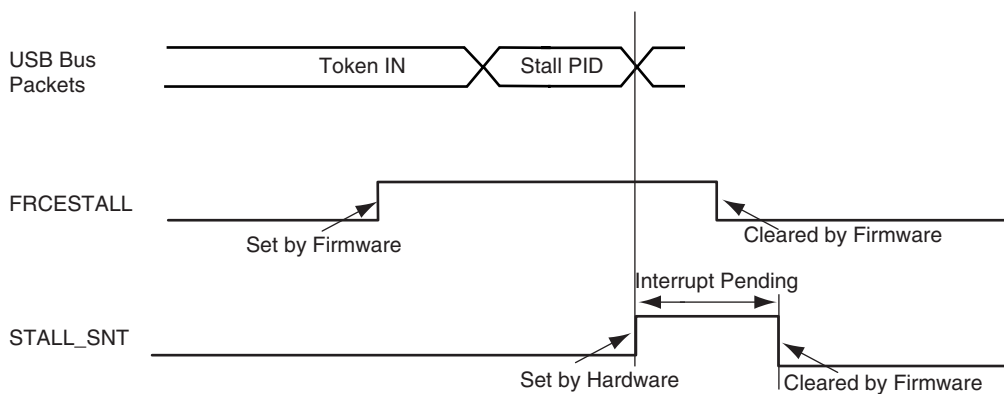
Figure 41-16. Stall Handshake Data IN Transfer
