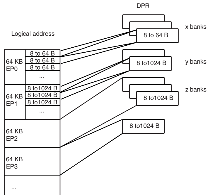
Figure 41-4. Logical Address Space for DPR Access:
