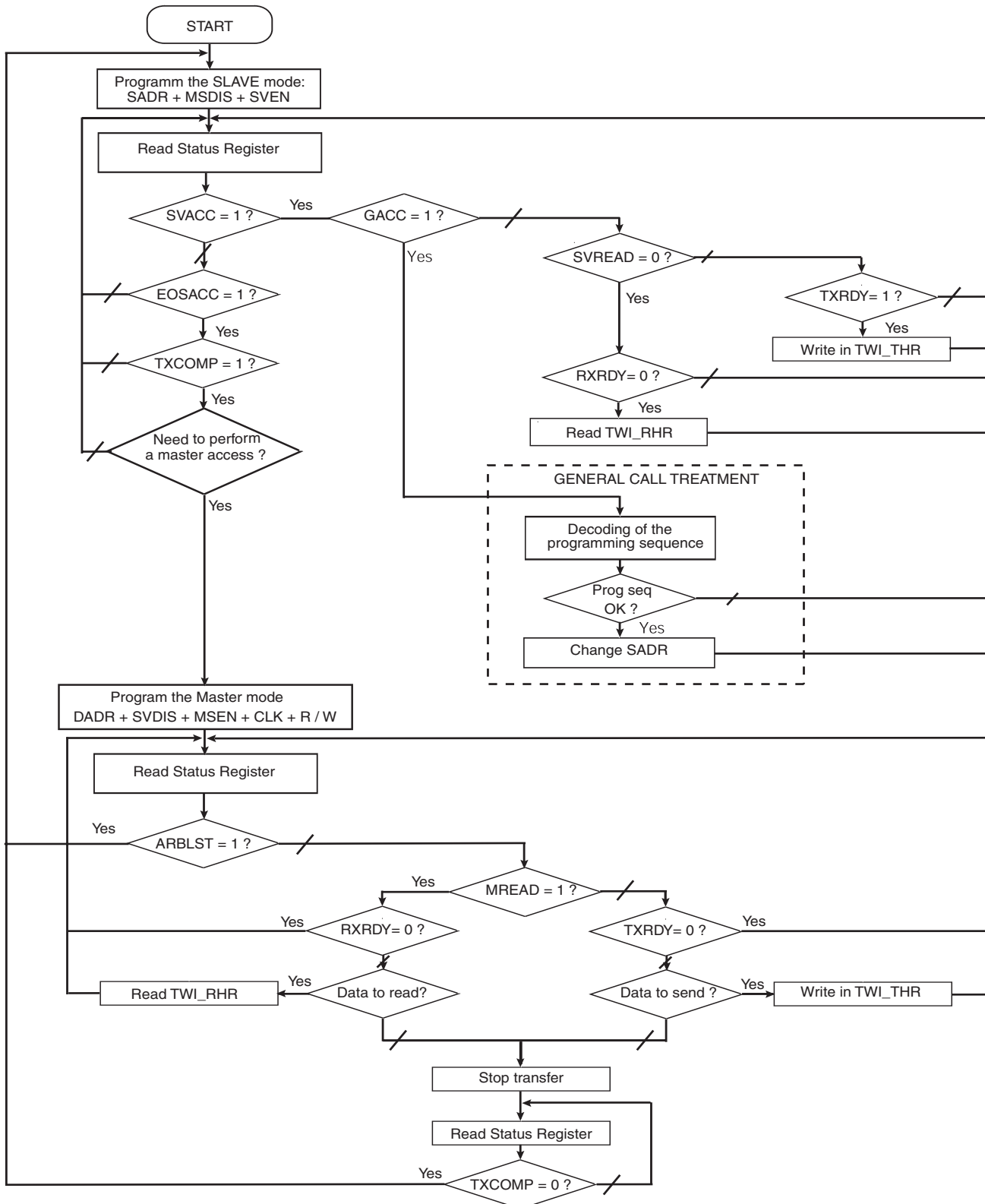
Figure 33-22. Multi-master Flowchart
