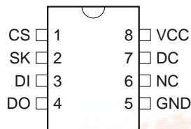
8-Pin PDIP
