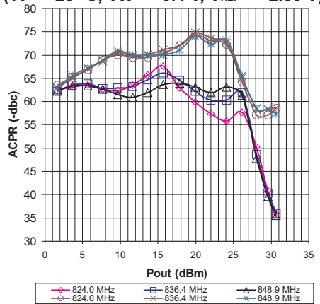
Figure 10: ACP1 and ACP2 vs. Output Power Over Frequency (T C = +25 °C, V CC = +3.4 V, V REF = +2.85 V)
