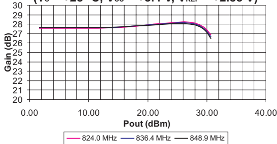
Figure 11: Large Signal Gain vs. Output Power Over Frequency (T C = +25 °C, V CC = +3.4 V, V REF = +2.85 V)
