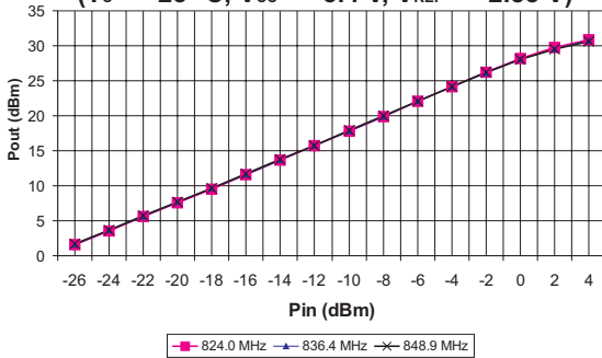
Figure 9: Input Power vs. Output Power Over Frequency (T C = +25 °C, V CC = +3.4 V, V REF = +2.85 V)
