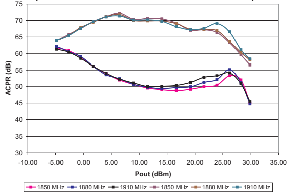
Figure 10: ACP1 & ACP2 vs. Output Power and Frequency (T C = +25 °C, V CC = +3.4 V, V REF = +2.9 V)
