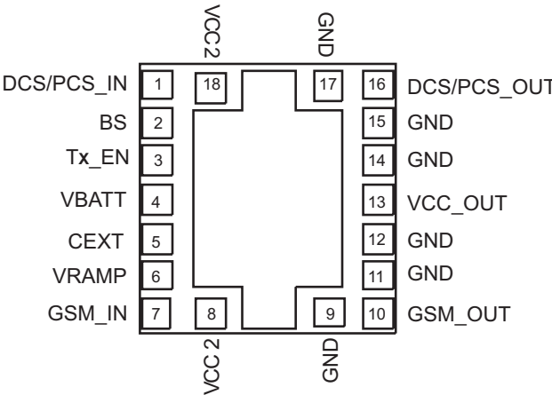
Figure 2: Pinout (X-ray Top View)
