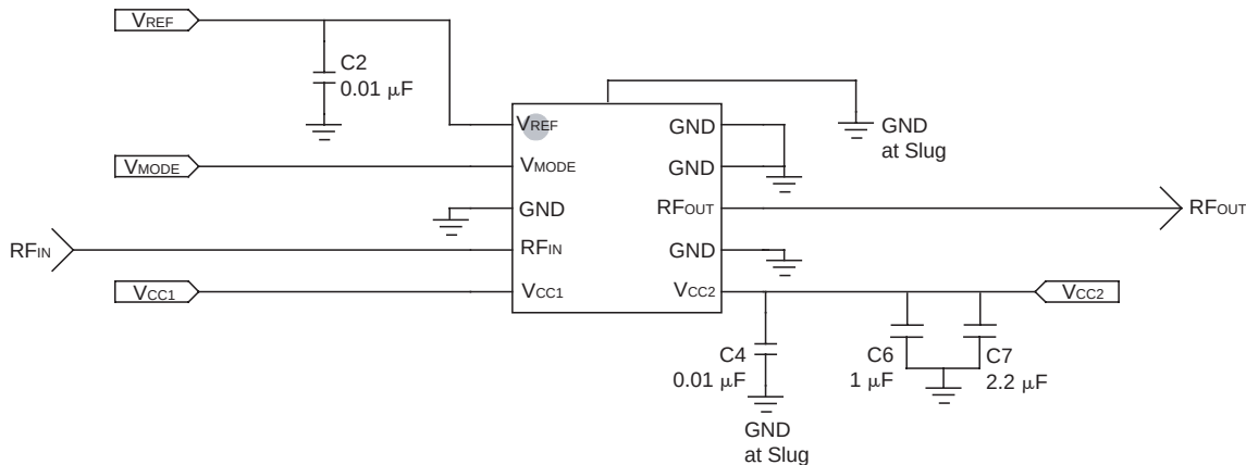
Figure 3: Application Schematic
