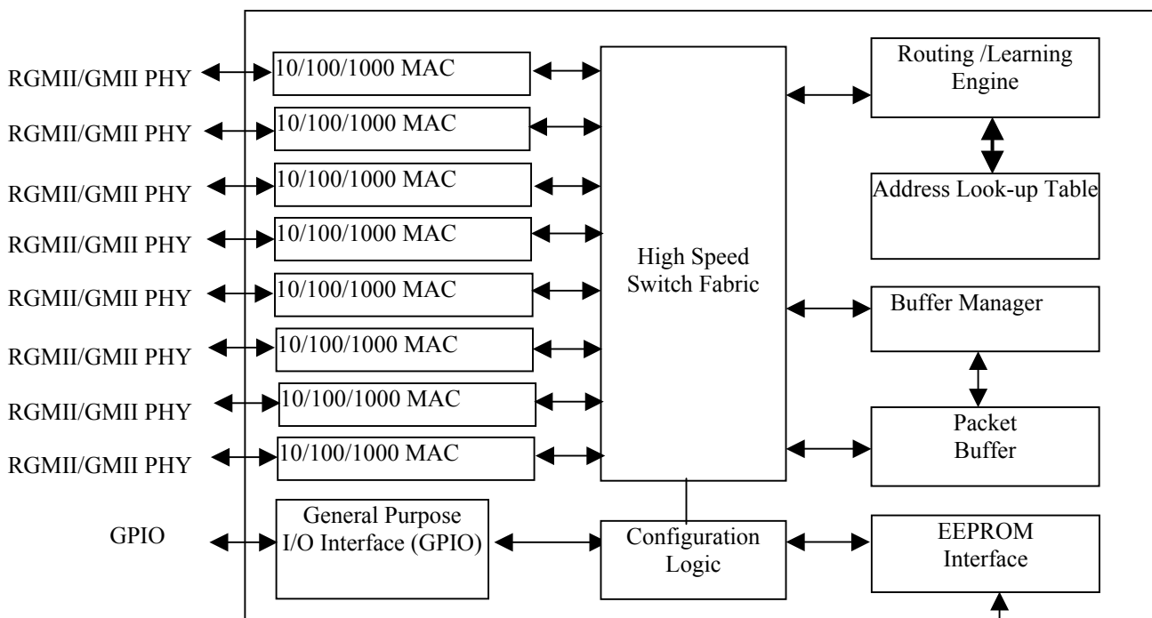
Fig-1 AX88658A Block Diagram
