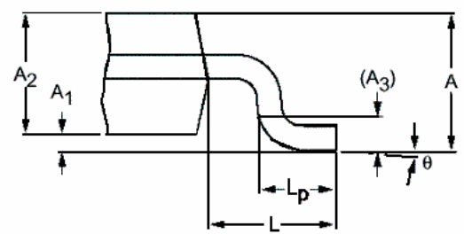
detail X
