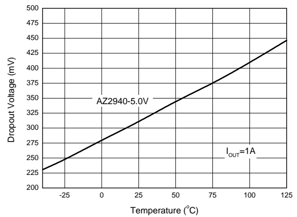
Figure 13. Dropout Voltage vs. Temperature
