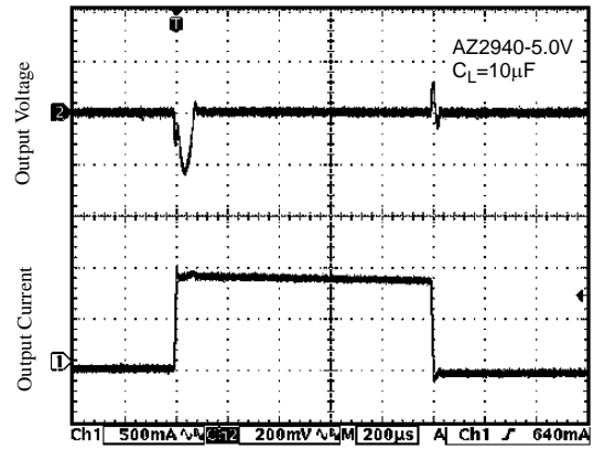
Figure 17. Load Transient
