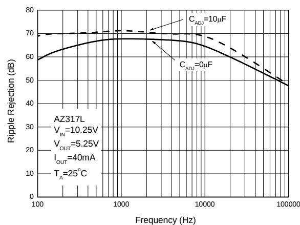
Figure 11. Ripple Rejection vs. Frequency
