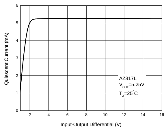
Figure 9. Minimum Operating Current
