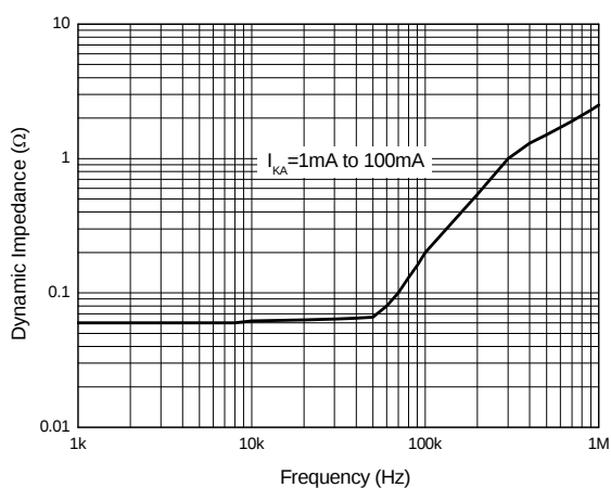
Figure 12. Dynamic Impedance vs. Frequency
