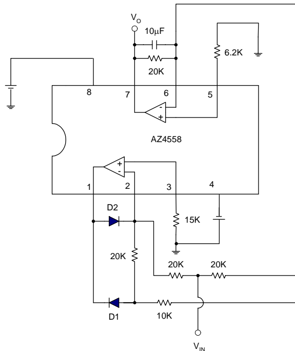
Figure 10. Application of AZ4558 in an AC/DC Converter
