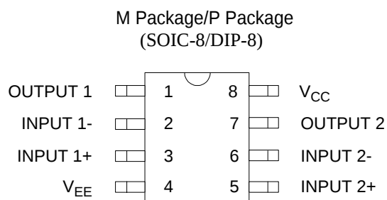
Figure 2. Pin Configuration of AZ4559 (Top View)
