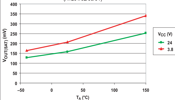
Output Voltage (On) versus Ambient Temperature (A1201/02/03/04)
