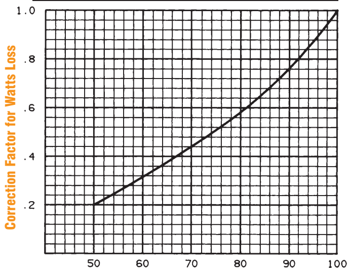
Watts Loss Correction vs. Percent Rated Current
