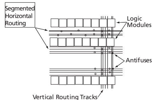
Figure 1-6 • MX Routing Structure
