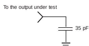
Load 1 (Used to measure propagation delay)
