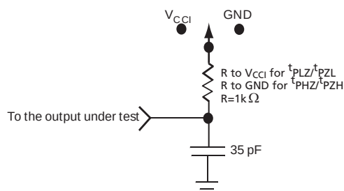
Load 2 (Used to measure rising/falling edges)
