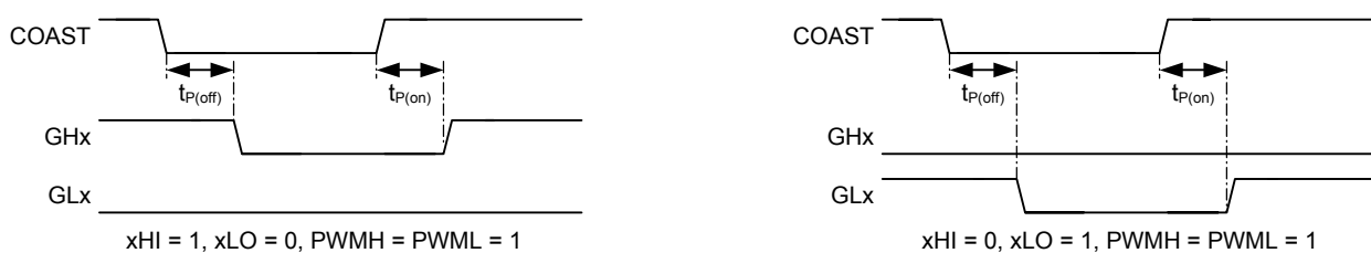
(C) Gate Drive Timing, COAST Inputs
