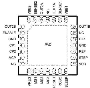
Pin-out Diagram
