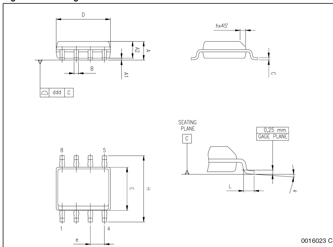
Figure 14. Package dimensions
