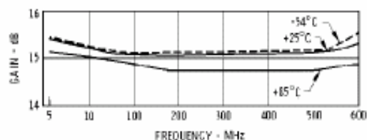
Gain
