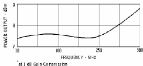
Power Output*
