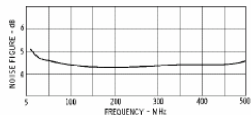
Noise Figure
