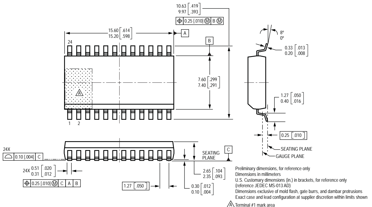
Package LW, 24-pin SOIC (A6279)
