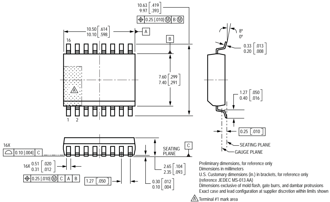
Package LW, 16-pin SOIC (A6278)
