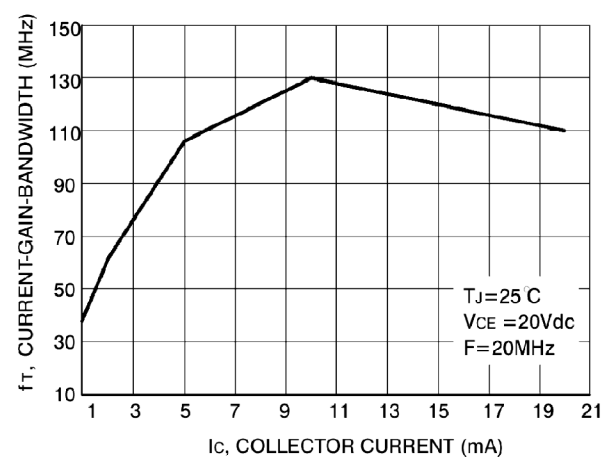
Current-Gain — Bandwidth
