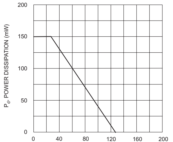
Fig. 4 Power Derating Curve, Total Package
