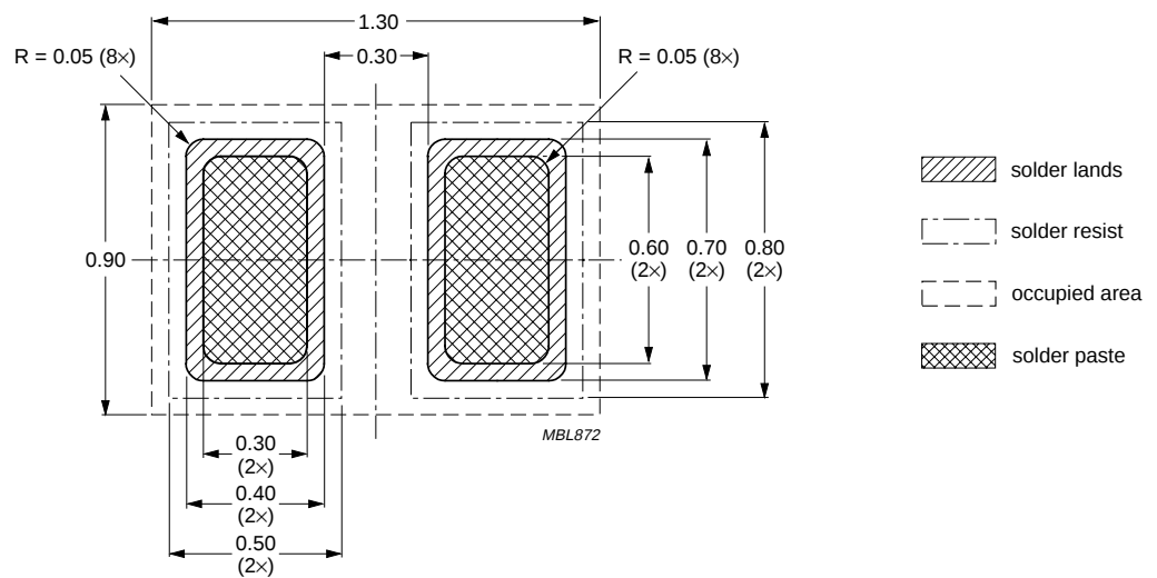
Fig 19. Reflow soldering footprint SOD123F
