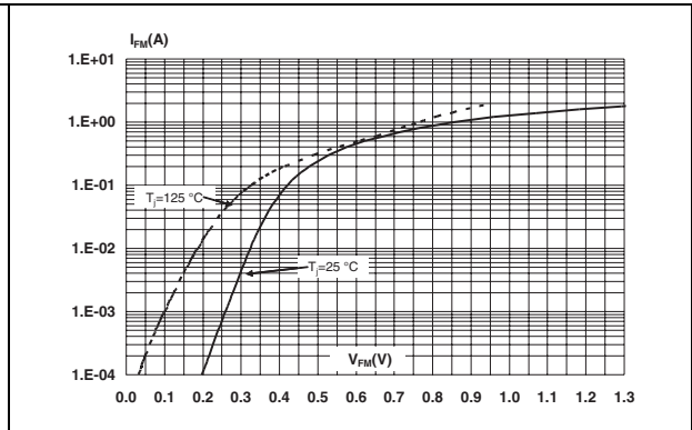
Figure 12. Forward voltage drop versus forward current (typical values)
