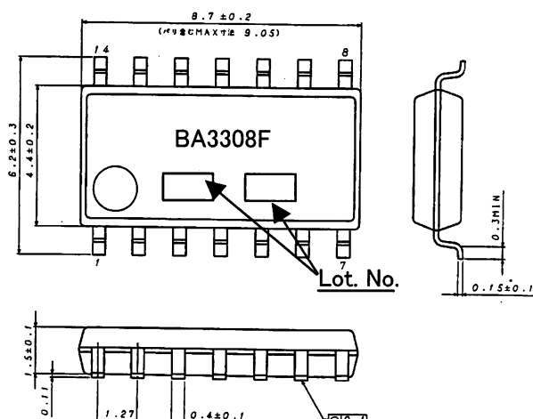
BA3308F: SOP14 (Unit: mm)
