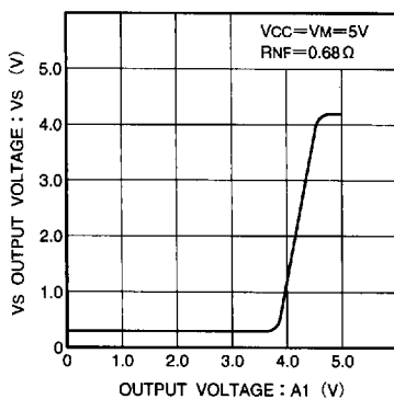
Fig.10 Vs output voltage vs. A1 output voltage
