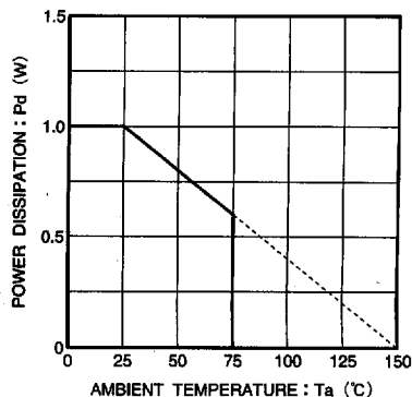
Fig.8 Power dissipation curve
