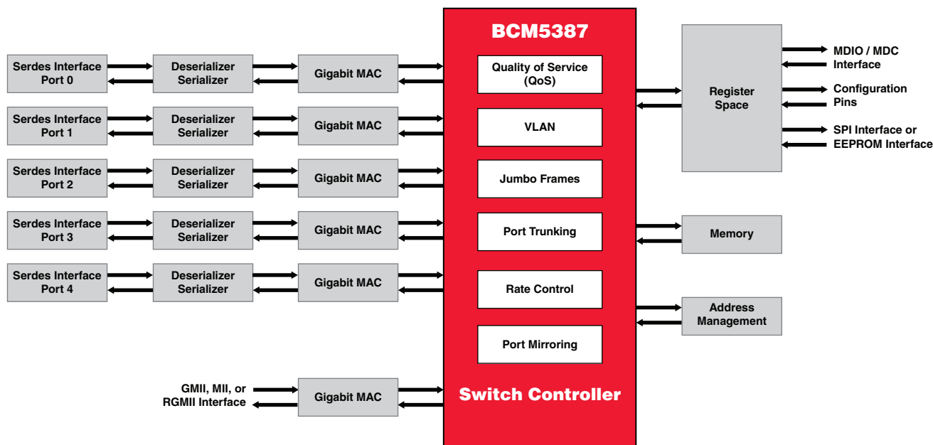
BCM5387 Block Diagram
