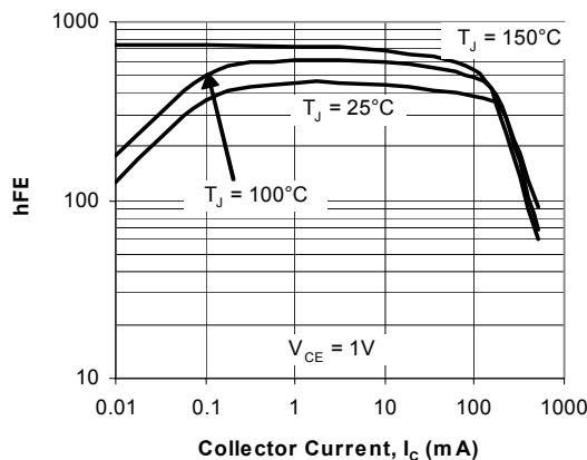
Fig. 1. BC337-16 Typical h_{FE} vs. I_C
